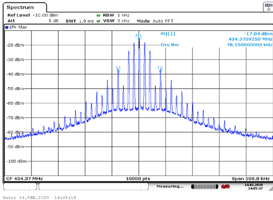
Plot 5: 99% bandwidth, 434.37 MHz
