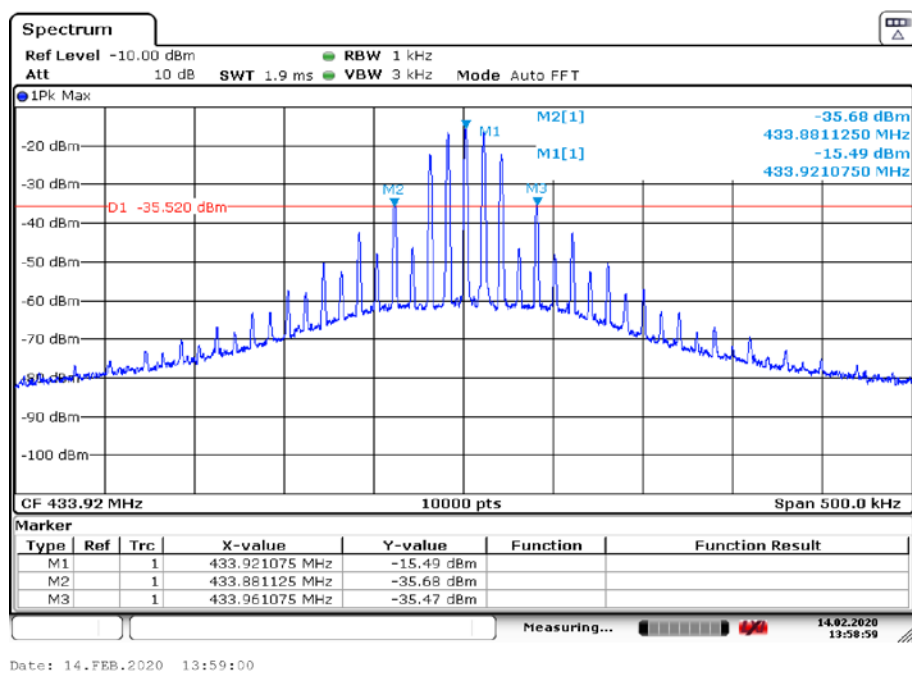
Plot 4: 20 dB bandwidth, 433.92 MHz
