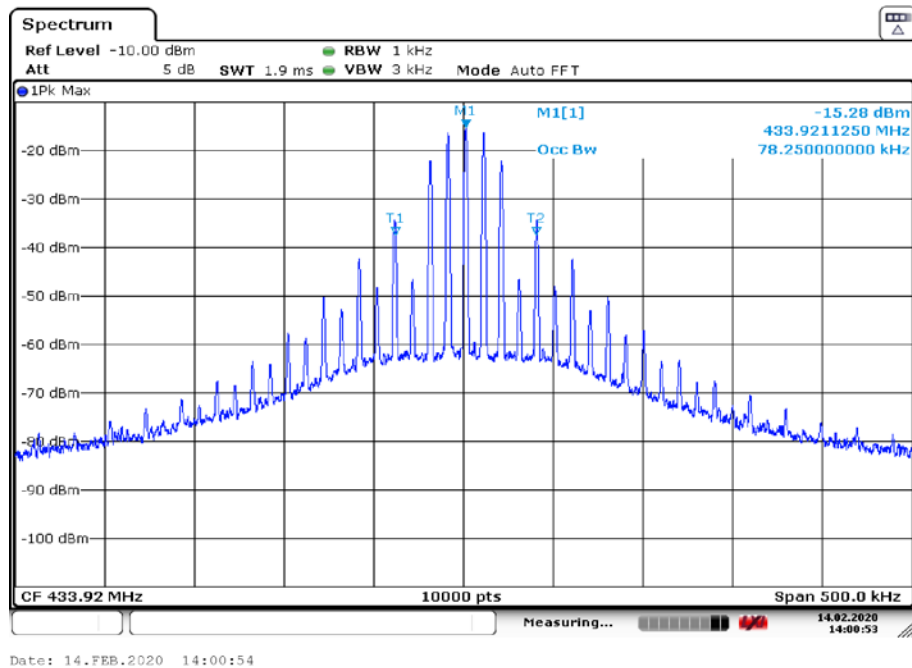
Plot 3: 99% bandwidth, 433.92 MHz
