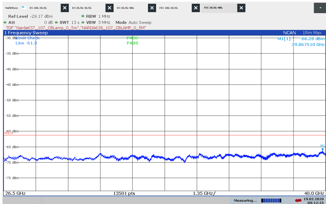
Plot 23: Max Hold on Channel A, 26.5 GHz to 40.0 GHz
