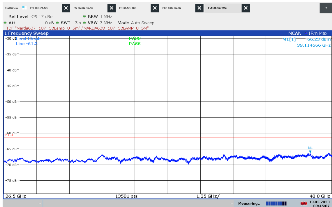
Plot 27: Max Hold on Channel C, 26.5 GHz to 40.0 GHz
