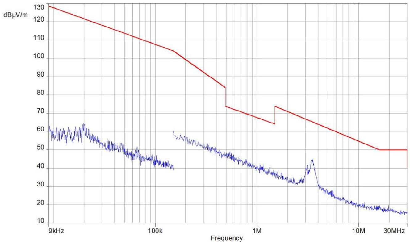
Plot 7: Channel A, 9 kHz to 30 MHz
