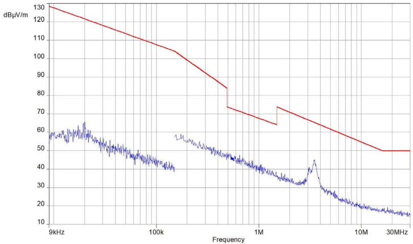
Plot 8: Channel B, 9 kHz to 30 MHz
