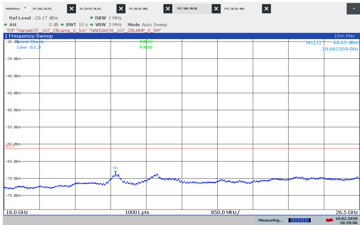
Plot 24: Max Hold on Channel B, 18 GHz to 26.5 GHz
