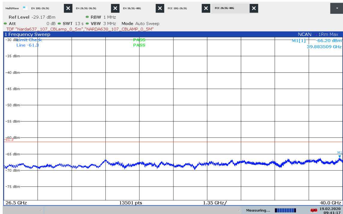
Plot 25: Max Hold on Channel B, 26.5 GHz to 40.0 GHz
