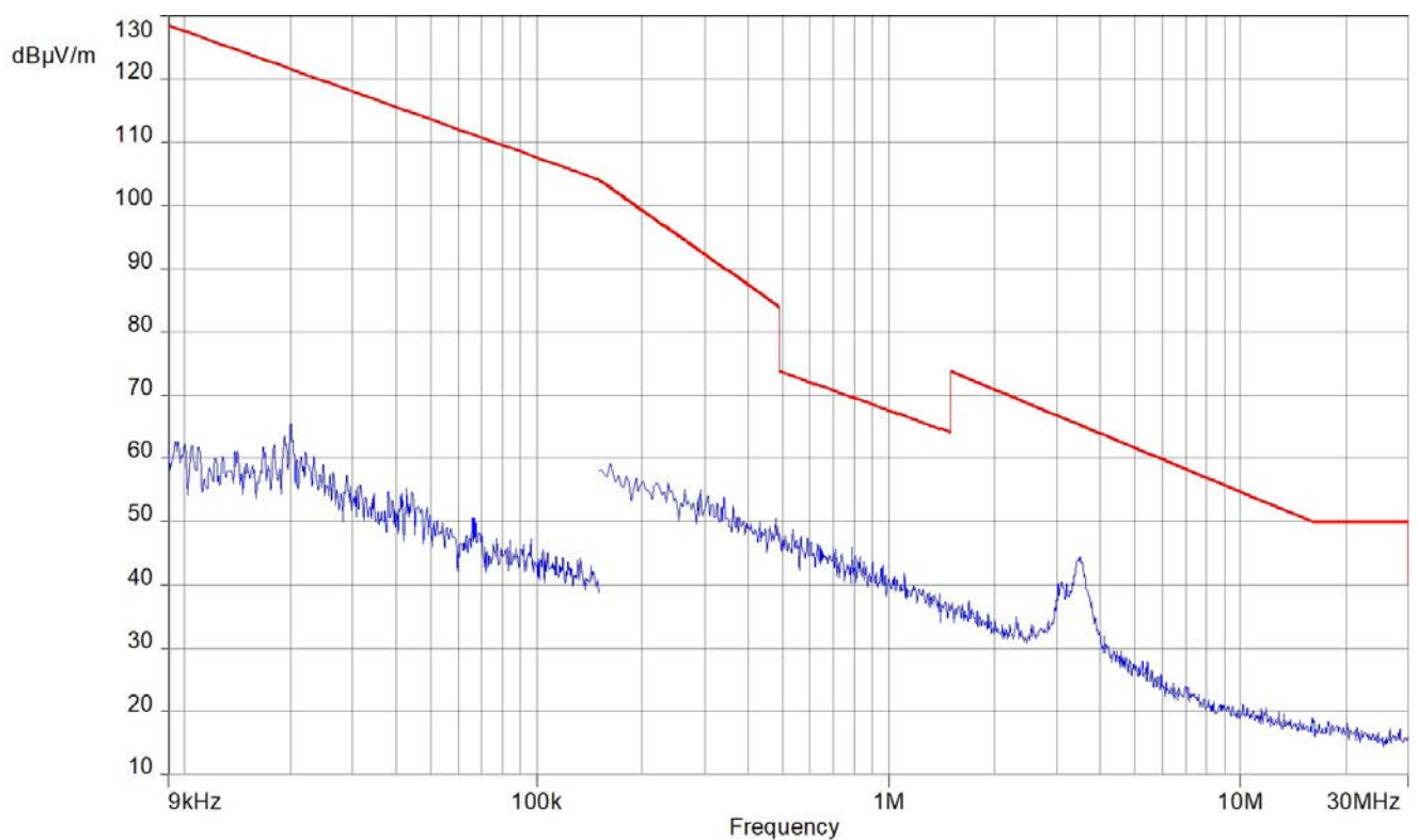
Plot 9: Channel C, 9 kHz to 30 MHz
