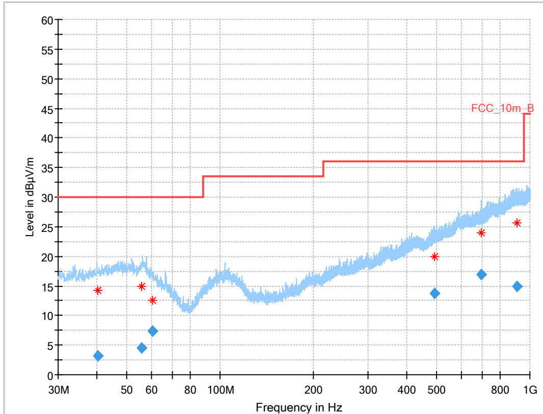
Plot 10: Channel A, 30 MHz to 1 GHz
