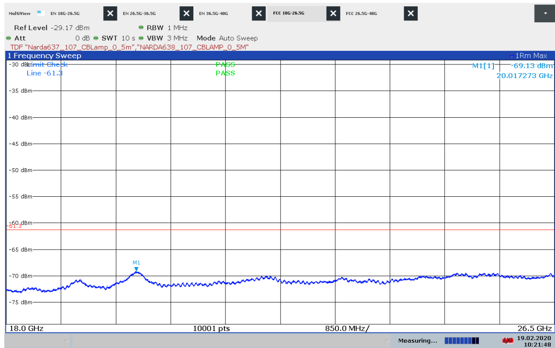
Plot 22: Max Hold on Channel A, 18 GHz to 26.5 GHz
