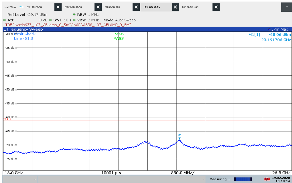
Plot 26: Max Hold on Channel C, 18 GHz to 26.5 GHz
