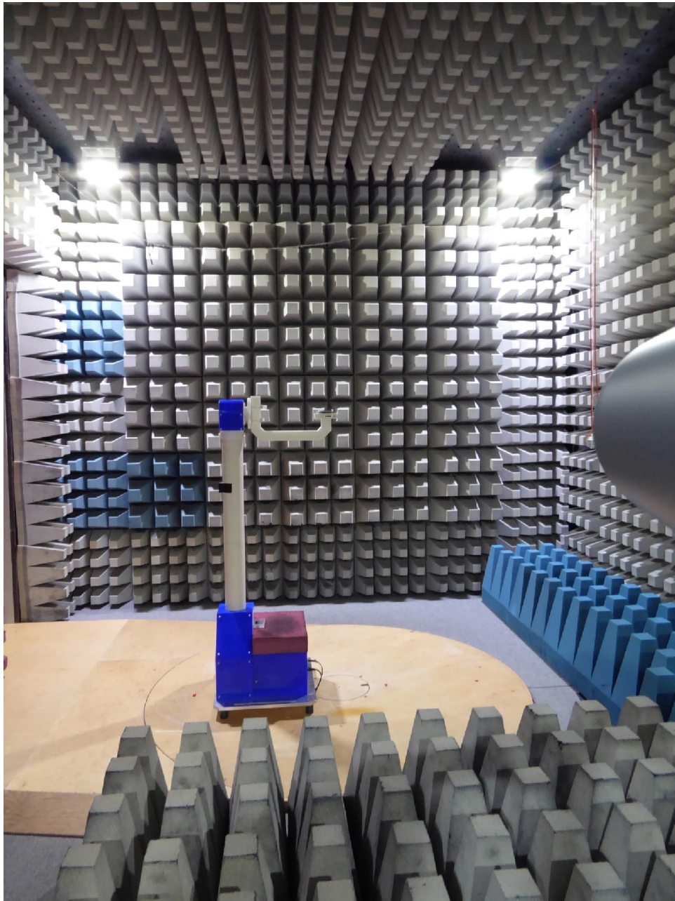
Test setup fully anechoic chamber (1 GHz to 5 GHz)
