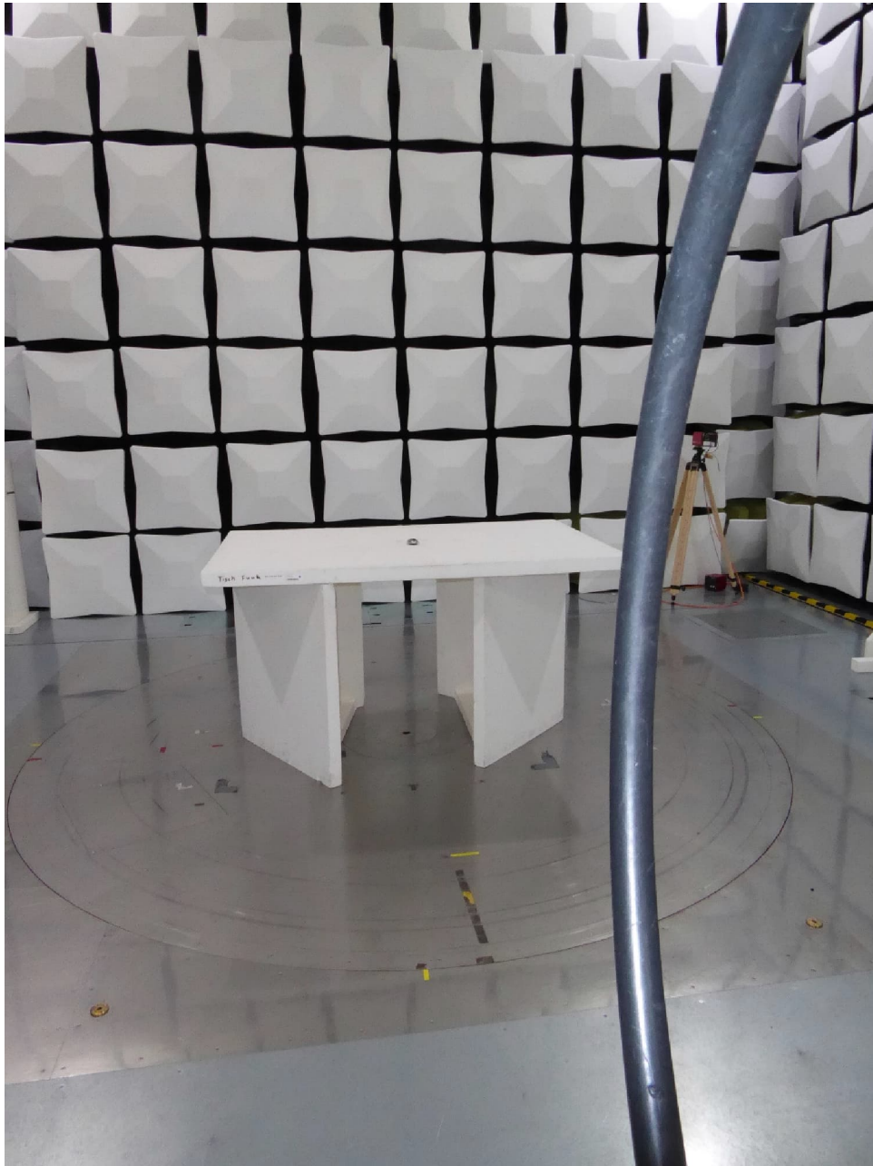
Test setup semi anechoic chamber (<30 MHz, position 1)
