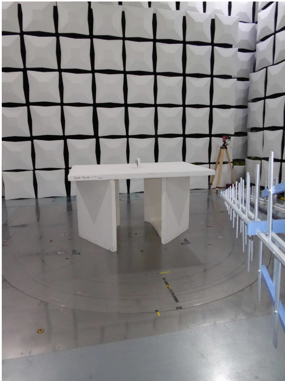
Test setup semi anechoic chamber (<1 GHz, position 3)
