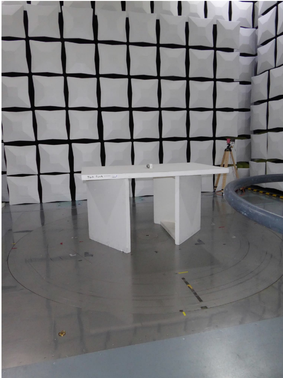
Test setup semi anechoic chamber (<30 MHz, position 2)
