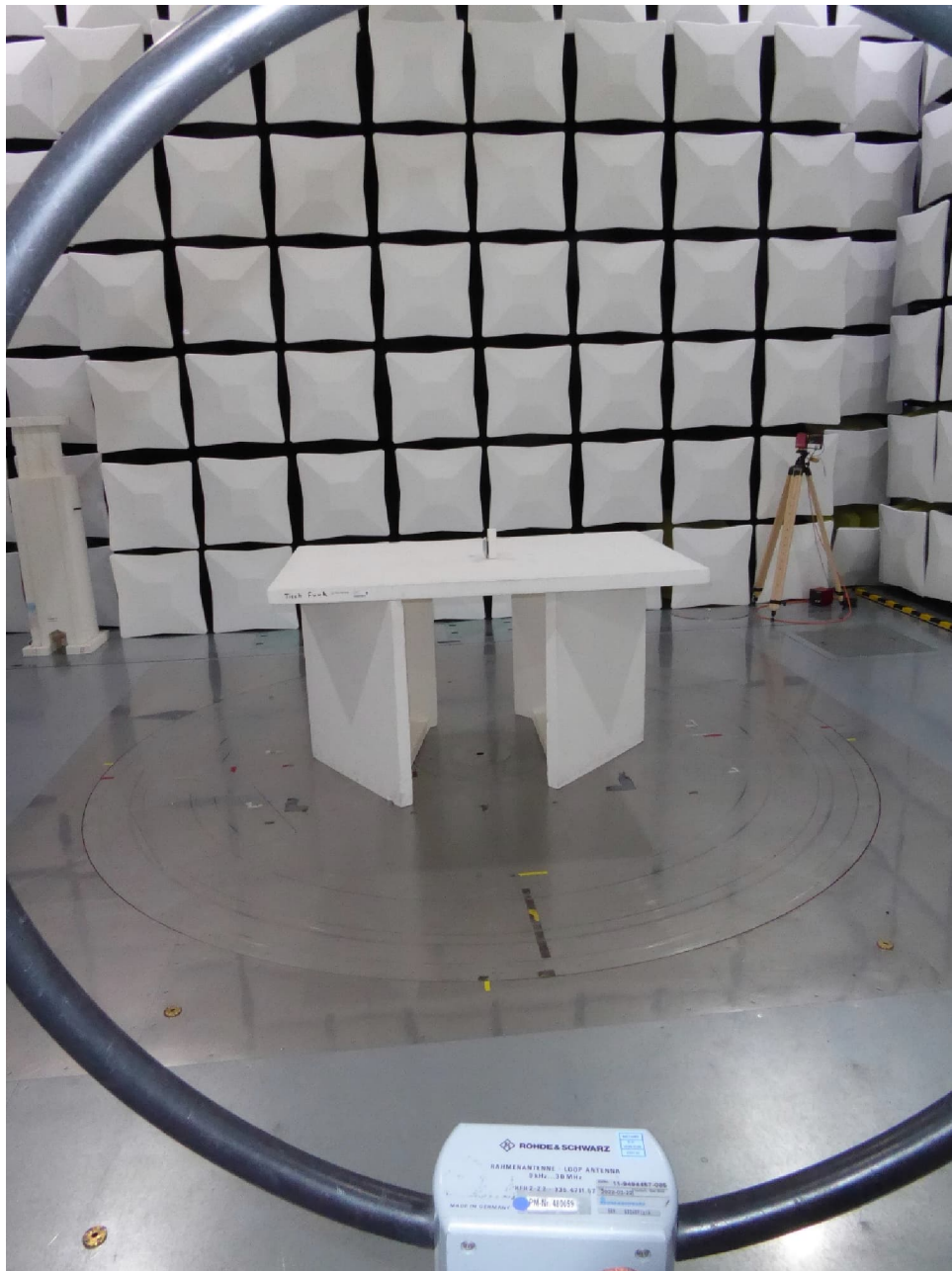
Test setup semi anechoic chamber (<30 MHz, position 3)
