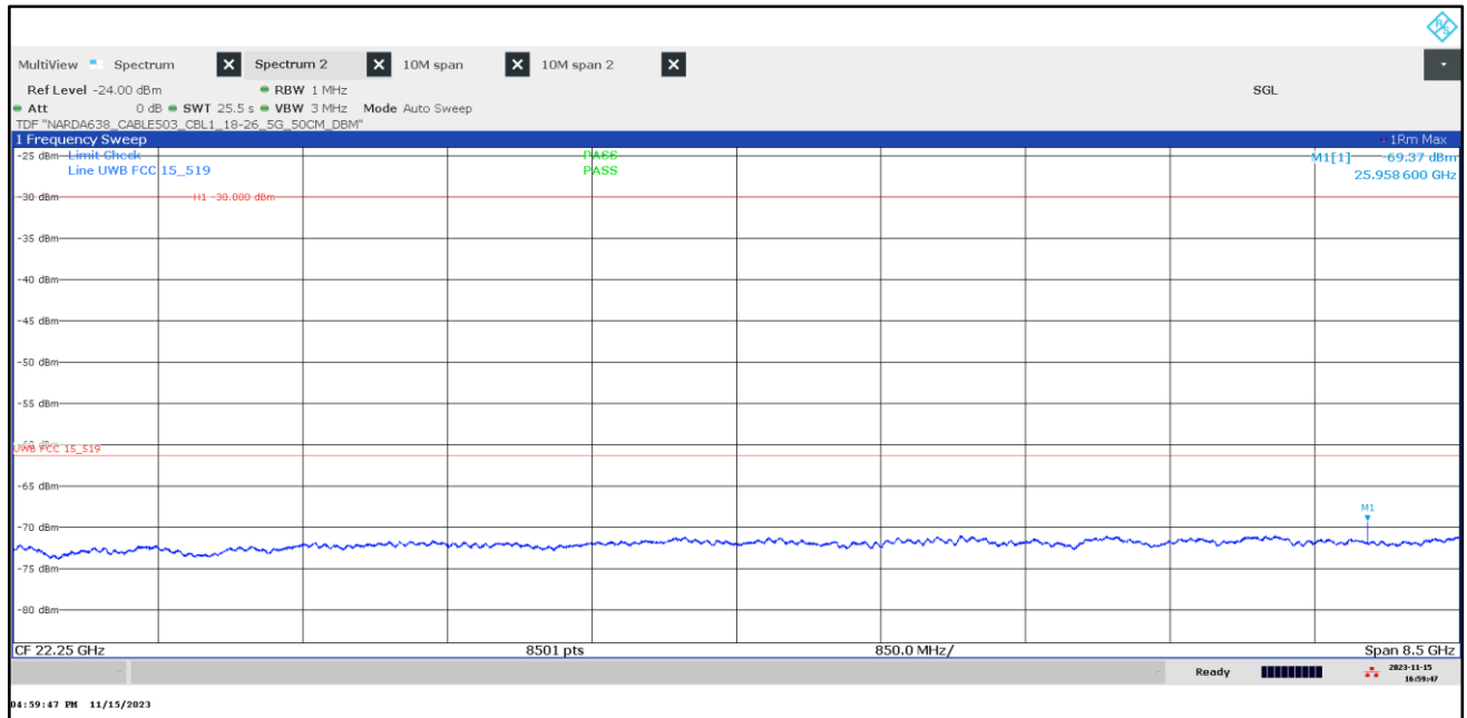
Plot 12: 18 GHz to 26.5 GHz, UWB test mode
