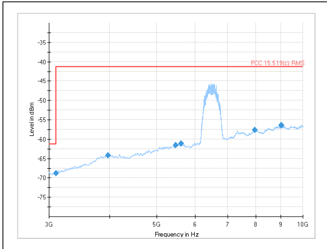
Plot 10: 3 GHz to 10 GHz, UWB test mode
