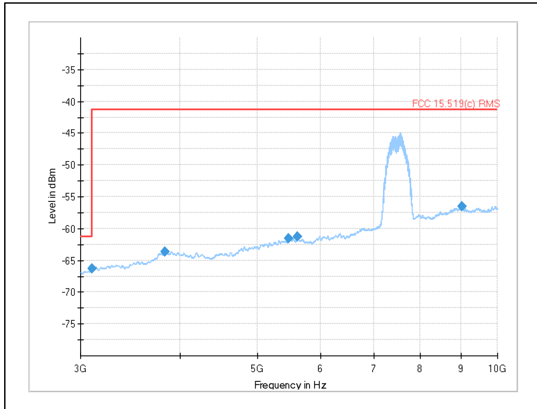
Plot 36: 3 GHz to 10 GHz, UWB test mode
