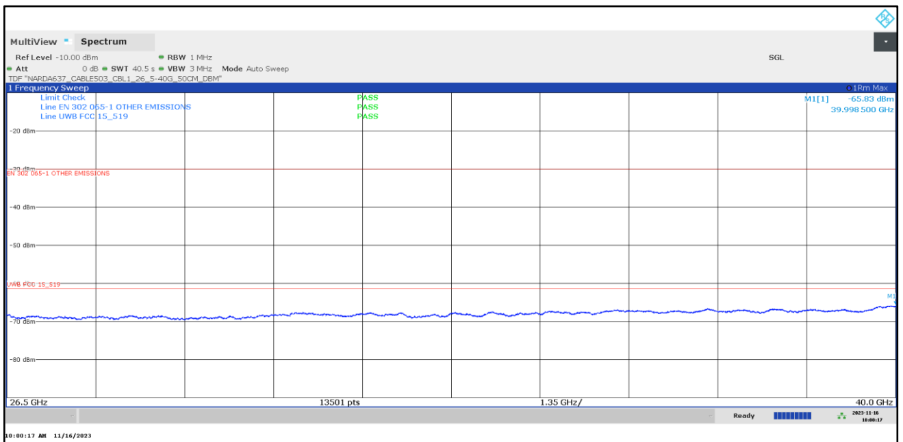
Plot 15: 26.5 GHz to 40.0 GHz, UWB test mode
