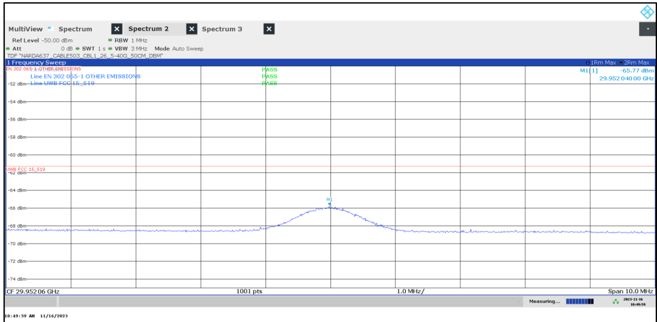
Plot 40: 29.9 GHz with 10 MHz span, UWB test mode
