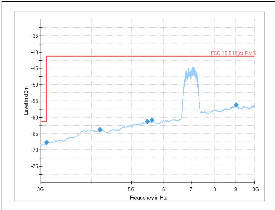
Plot 23: 3 GHz to 10 GHz, UWB test mode
