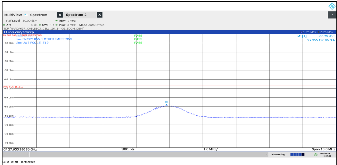
Plot 27: 27.9 GHz with 10 MHz span, UWB test mode
