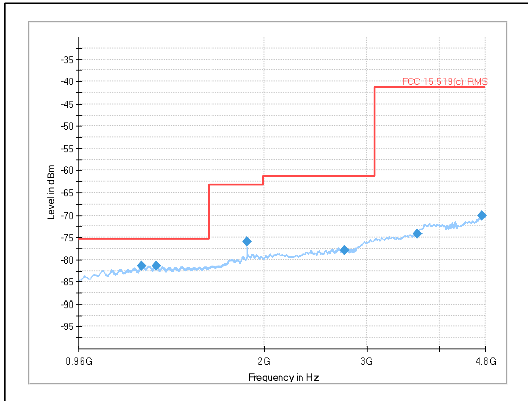
Plot 48: 960 MHz to 4.8 GHz (Limit acc. to §15.519 (c)), UWB test mode
