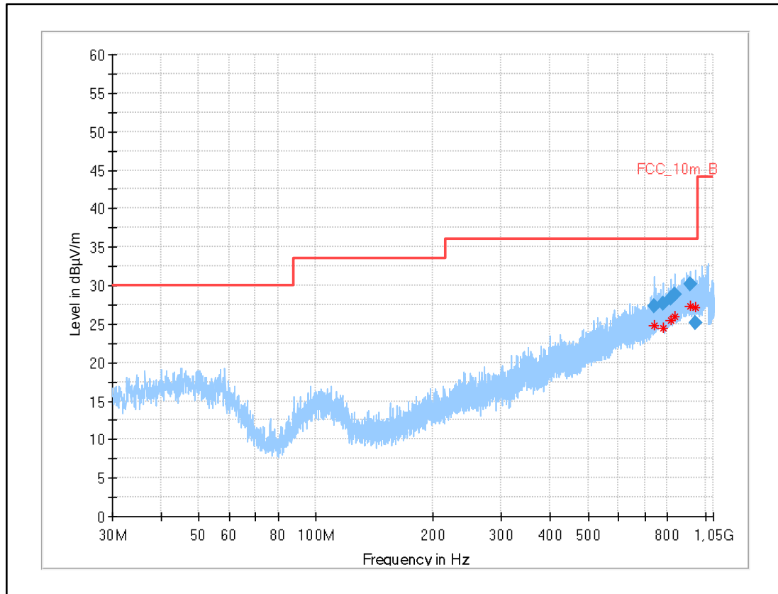
Plot 8: 30 MHz to 1 GHz, UWB test mode
