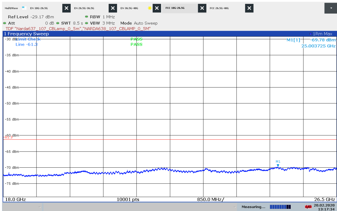
Plot 32: Max Hold on Channel C, 18 GHz to 26.5 GHz
