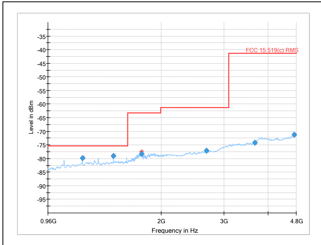
Plot 9: 960 MHz to 4.8 GHz (Limit acc. to §15.519 (c)), UWB test mode
