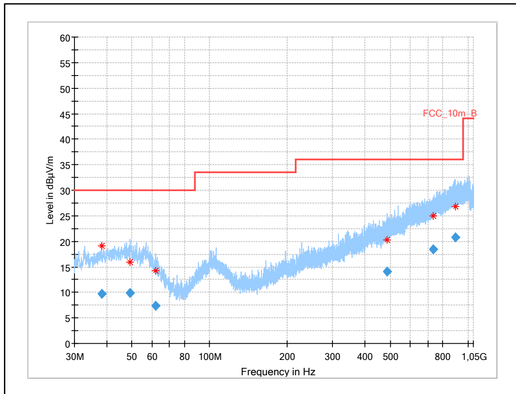
Plot 47: 30 MHz to 1 GHz, UWB test mode
