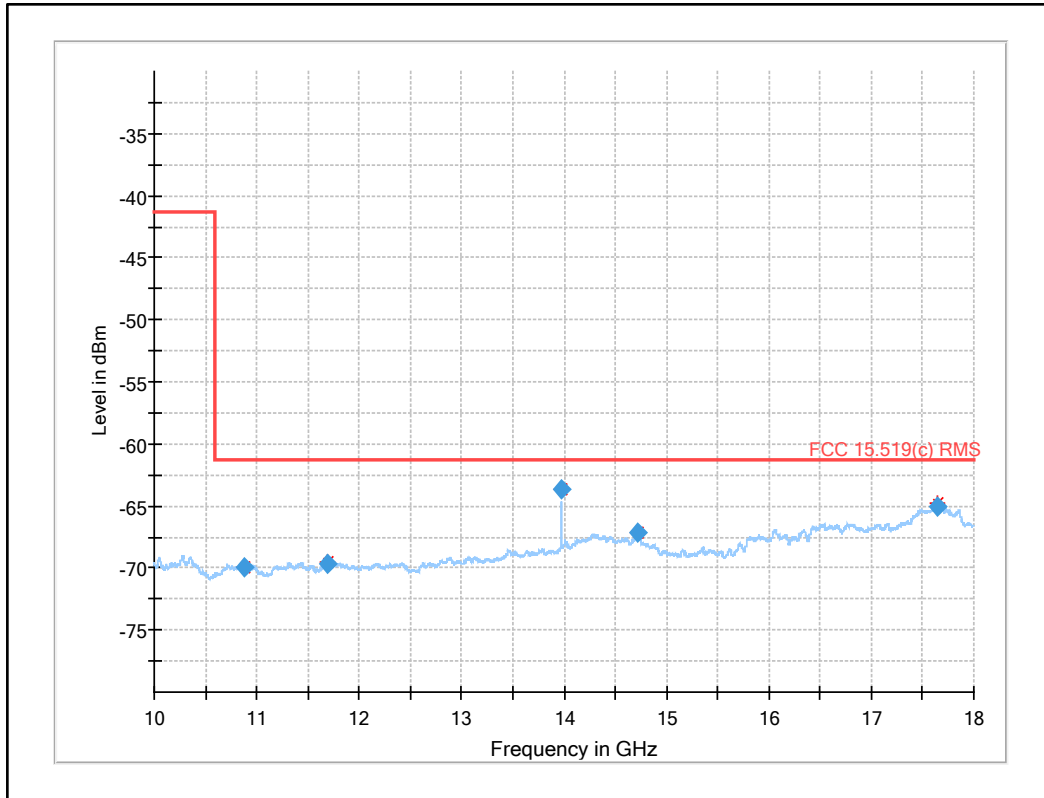
Plot 24: 10 GHz to 18 GHz, UWB test mode
