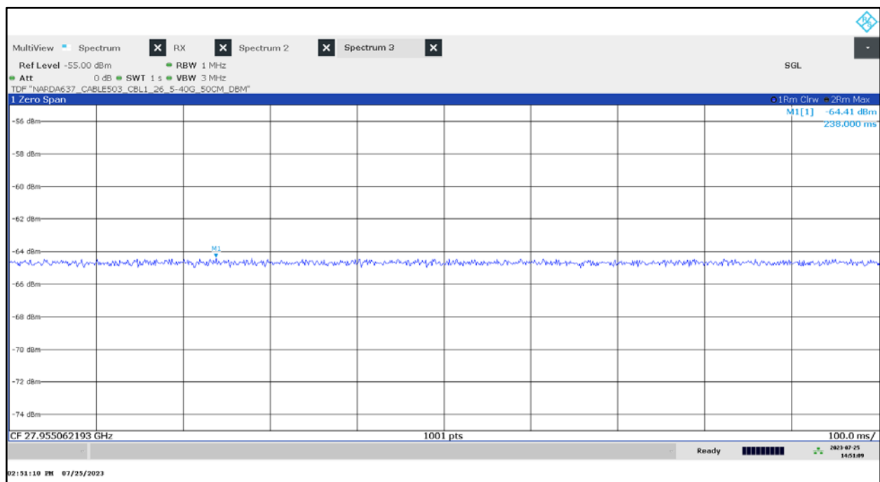
Plot 28: 27.9 GHz, UWB test mode zero span
