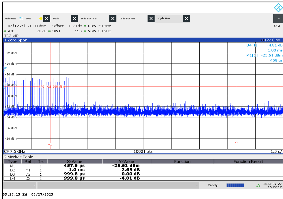
Plot 59: Emissions of the EUT, only at the beginning with associated receiver (Normal mode CH8)
