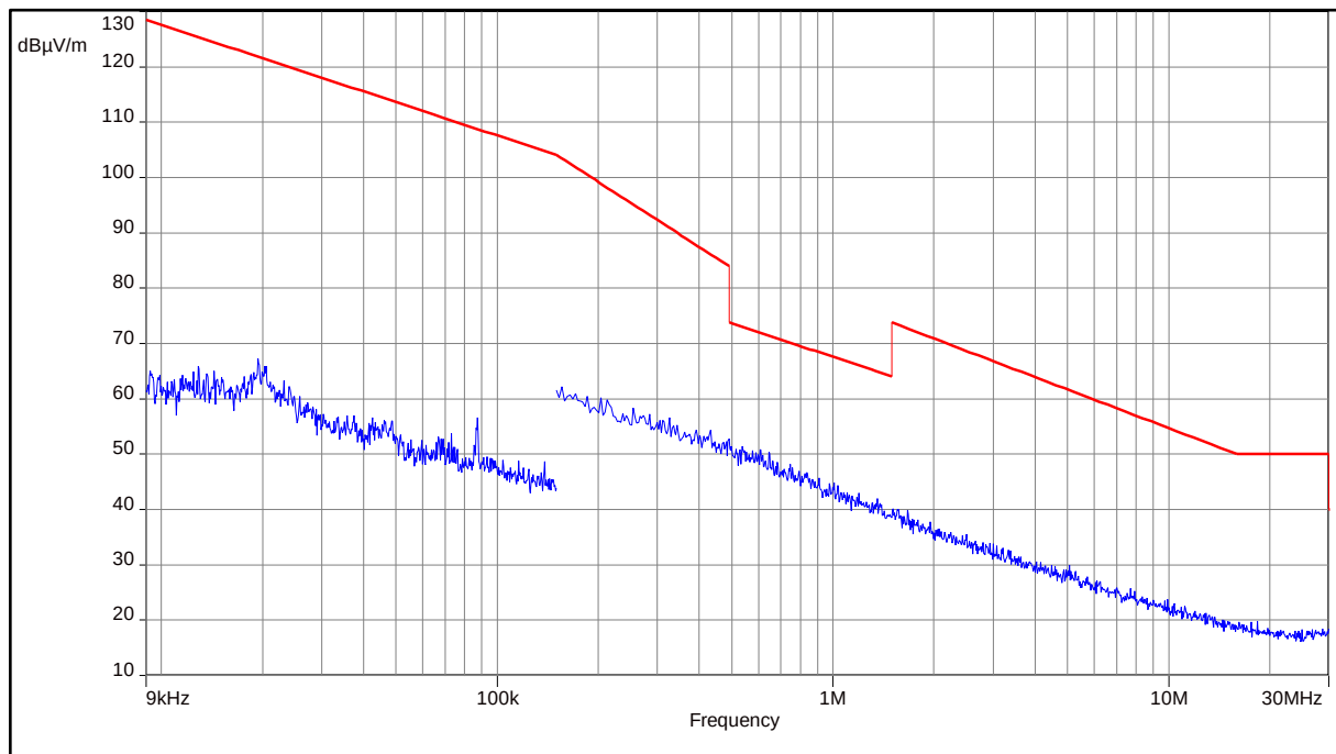
Plot 33: 9 kHz to 30 MHz, UWB test mode
