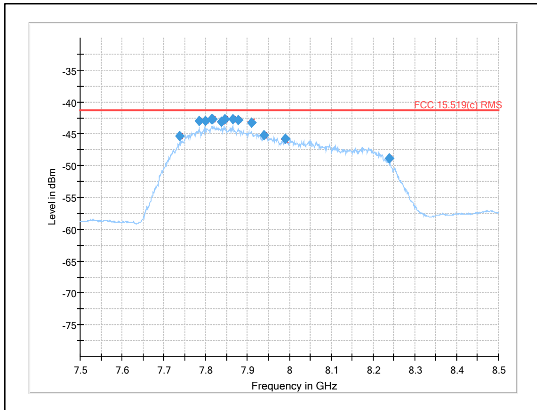
Plot 44: Fundamental emission (UWB test mode): RMS
