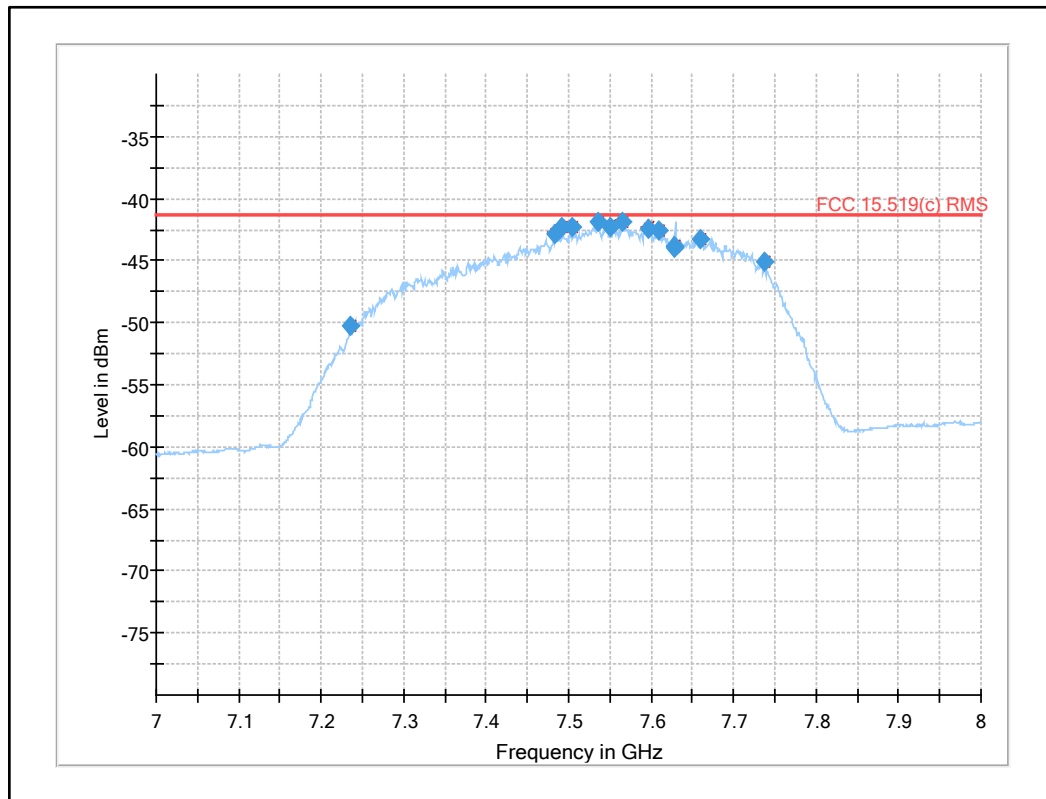
Plot 31: Fundamental emission (UWB test mode): RMS
