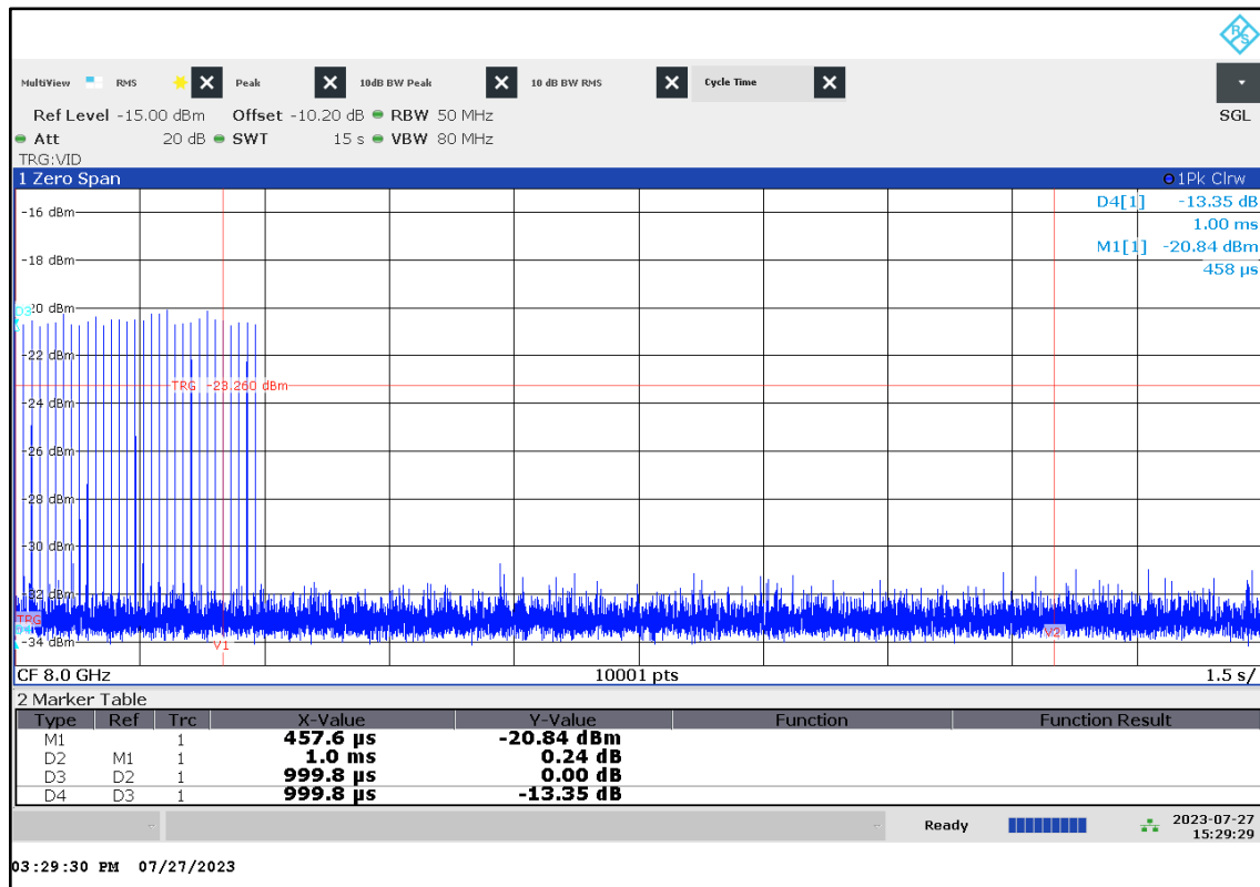
Plot 60: Emissions of the EUT, only at the beginning with associated receiver (Normal mode CH9)
