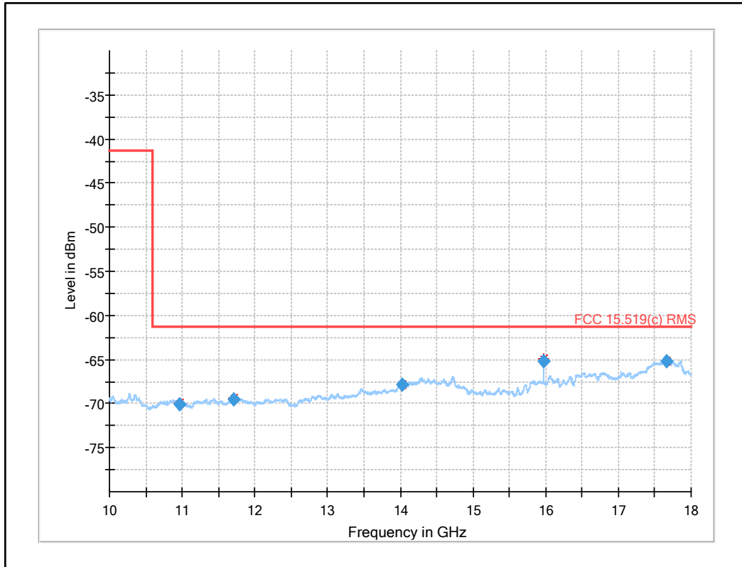
Plot 50: 10 GHz to 18 GHz, UWB test mode
