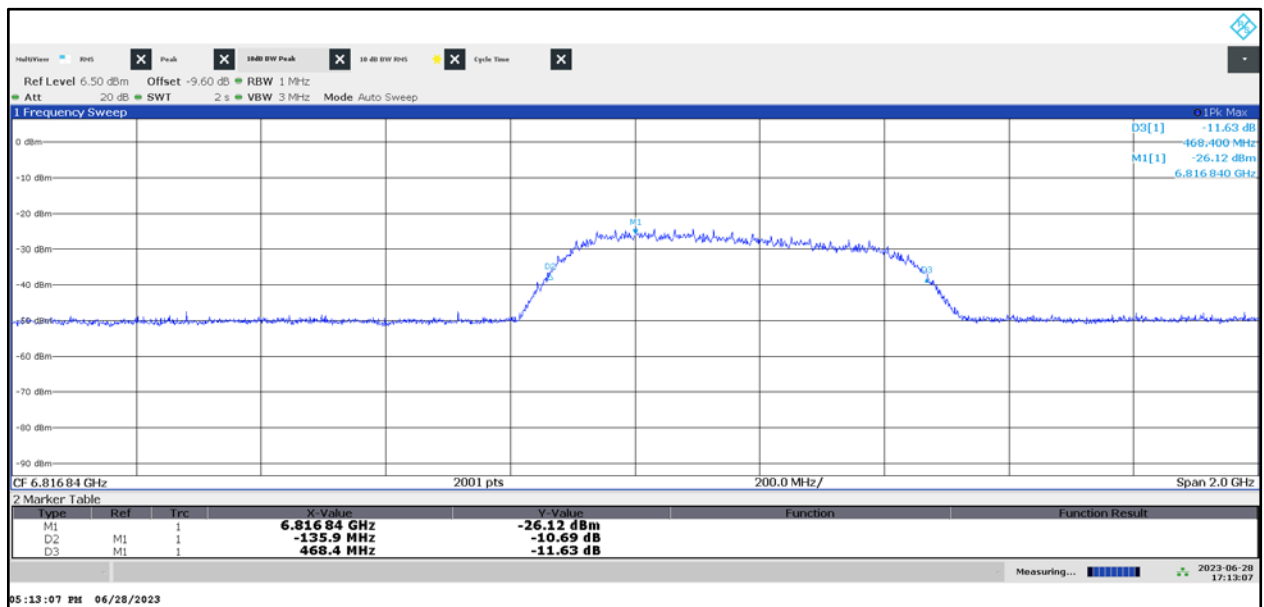
Plot 2: 10 dB bandwidth, UWB test mode channel 6
