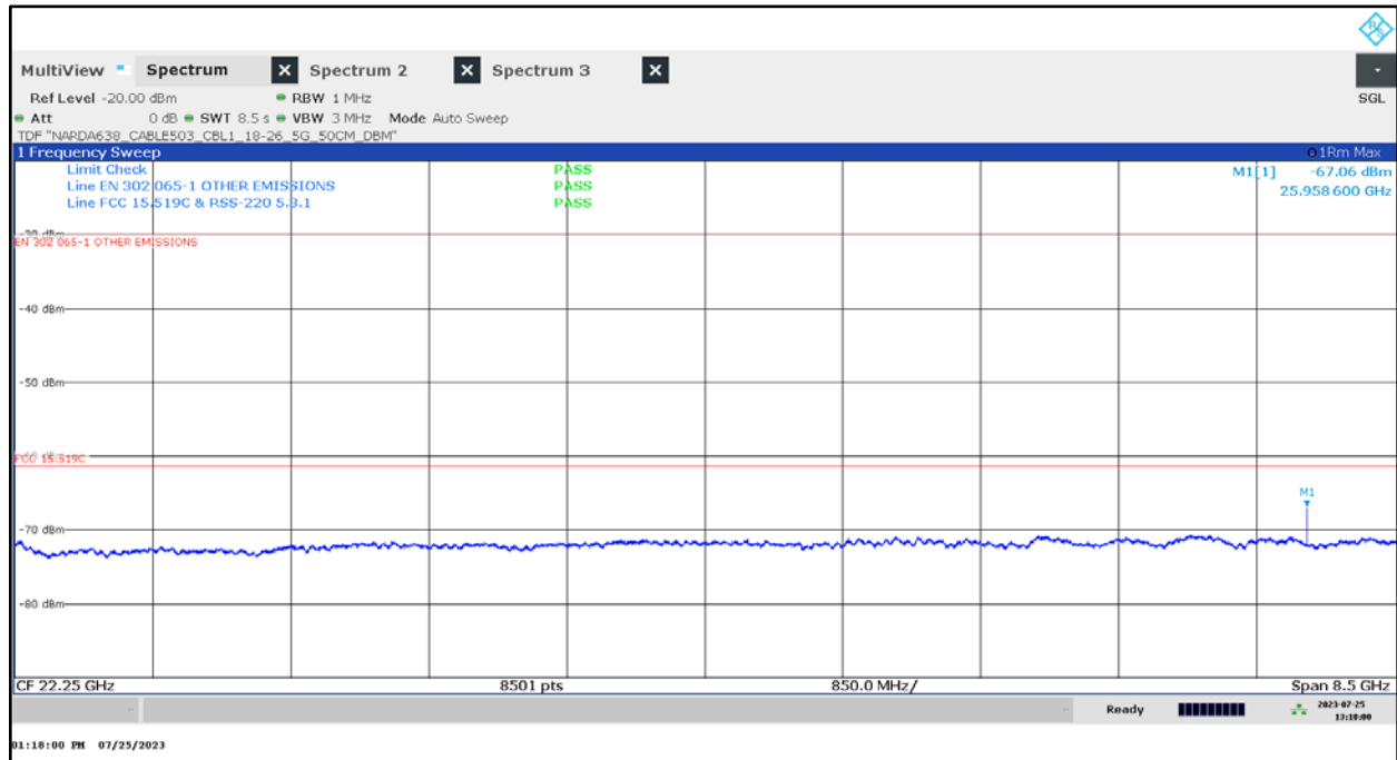
Plot 12: 18 GHz to 26.5 GHz, UWB test mode
