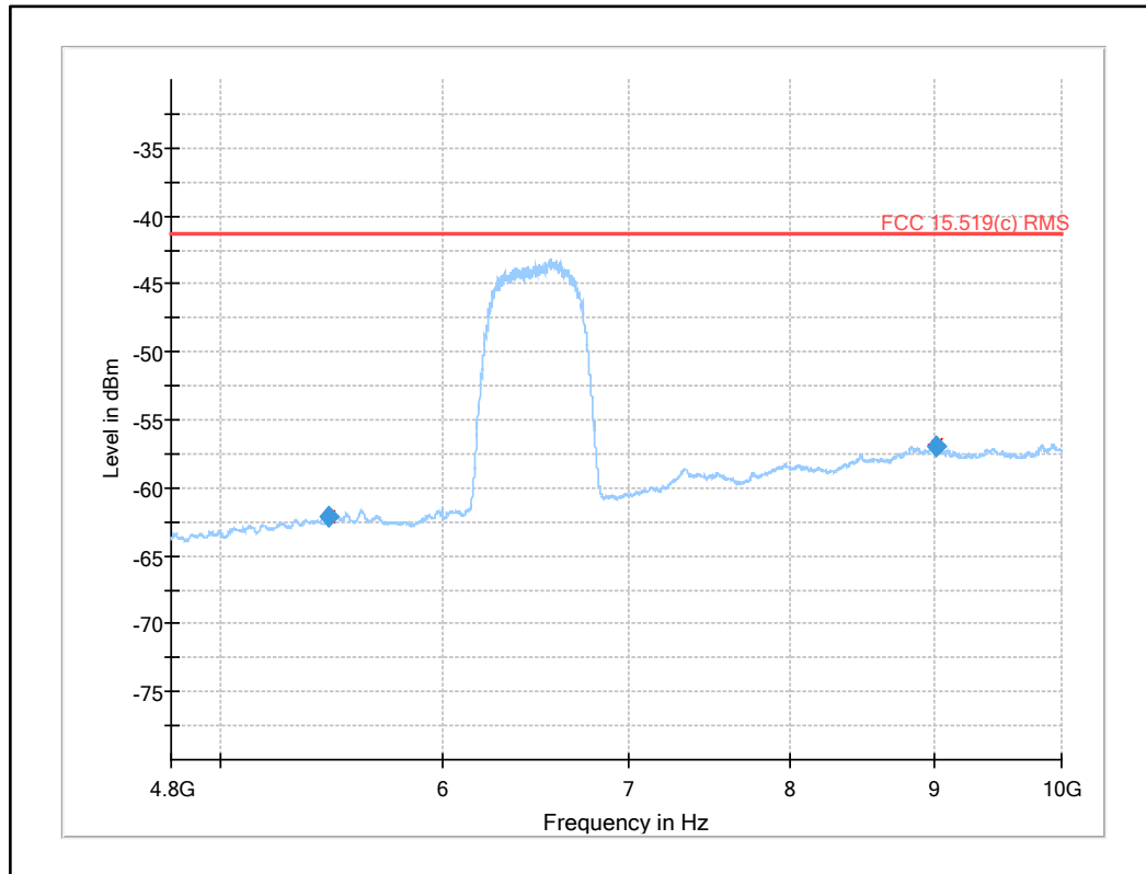
Plot 10: 4.8 GHz to 10 GHz, UWB test mode
