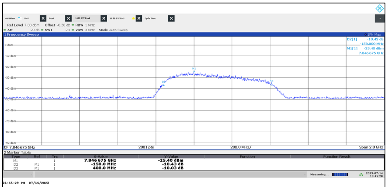
Plot 4: 10 dB bandwidth, UWB test mode channel 9
