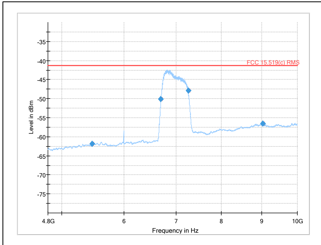
Plot 23: 4.8 GHz to 10 GHz, UWB test mode
