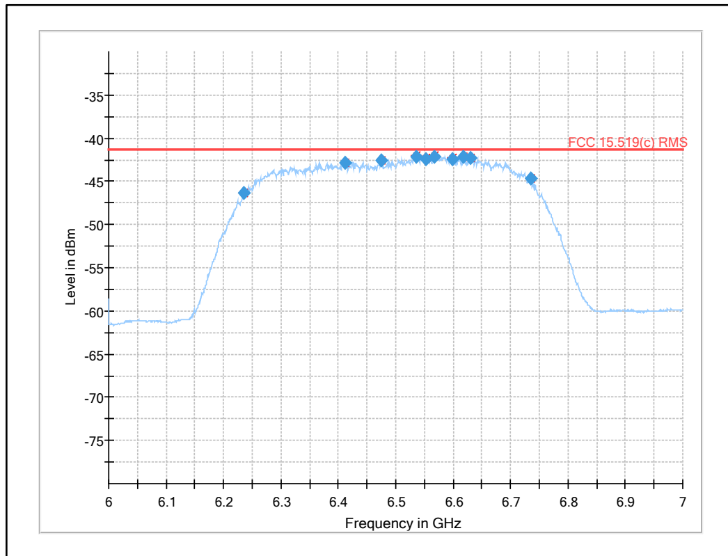
Plot 5: Fundamental emission (UWB test mode): RMS
