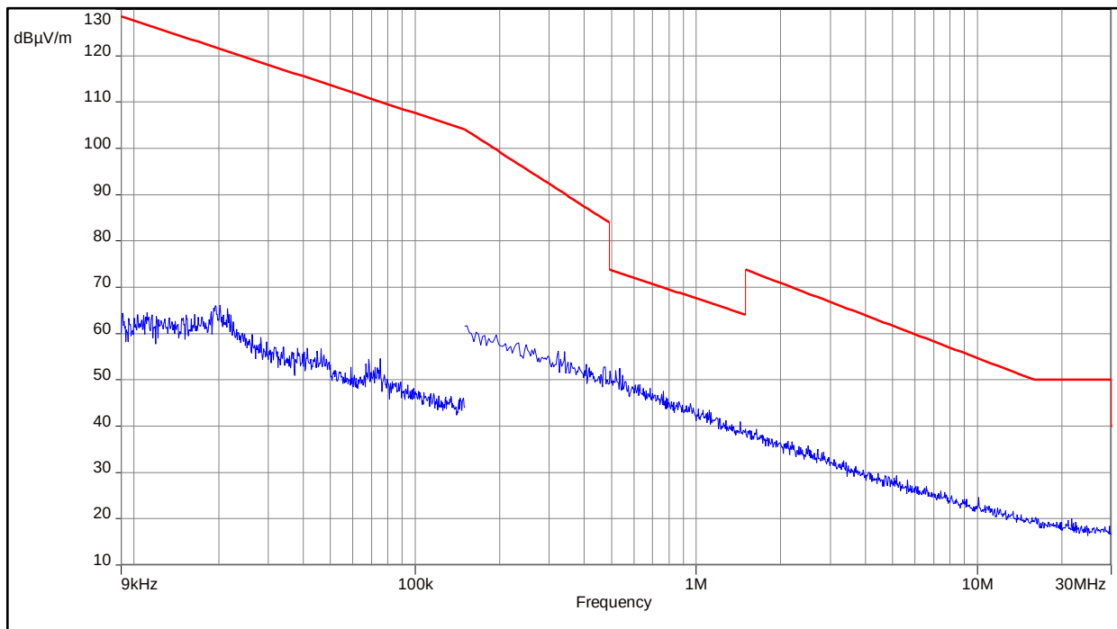
Plot 20: 9 kHz to 30 MHz, UWB test mode
