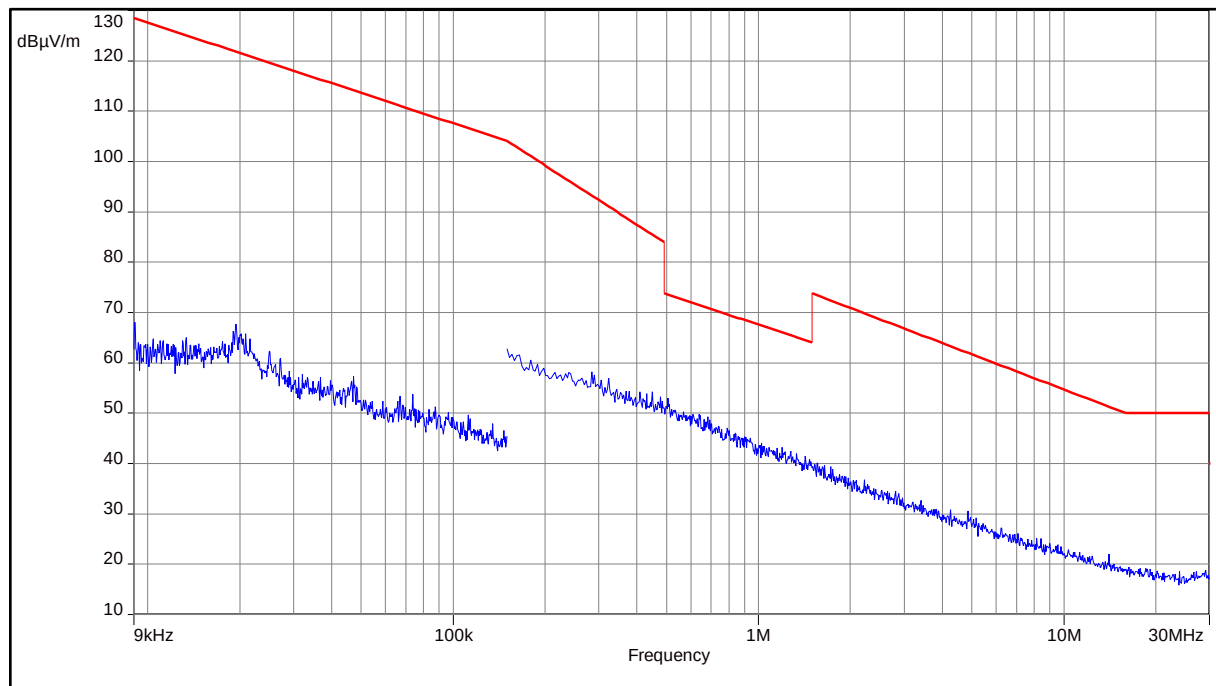
Plot 46: 9 kHz to 30 MHz, UWB test mode
