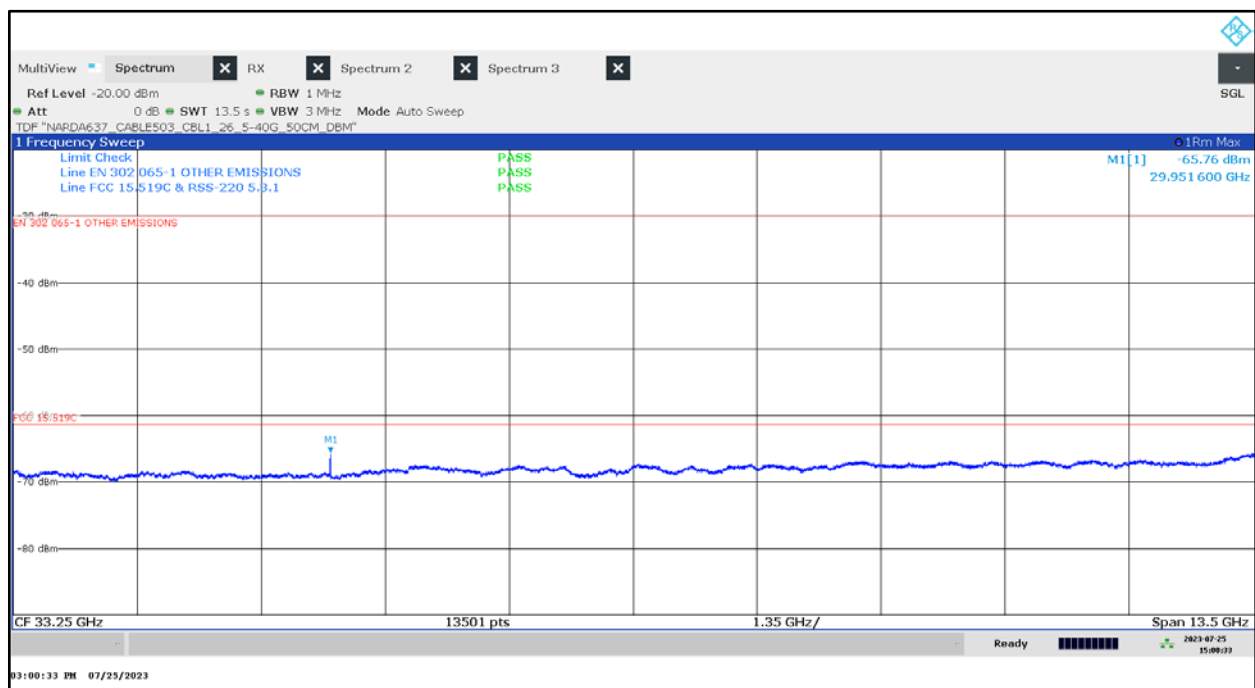
Plot 39: 26.5 GHz to 40.0 GHz, UWB test mode
