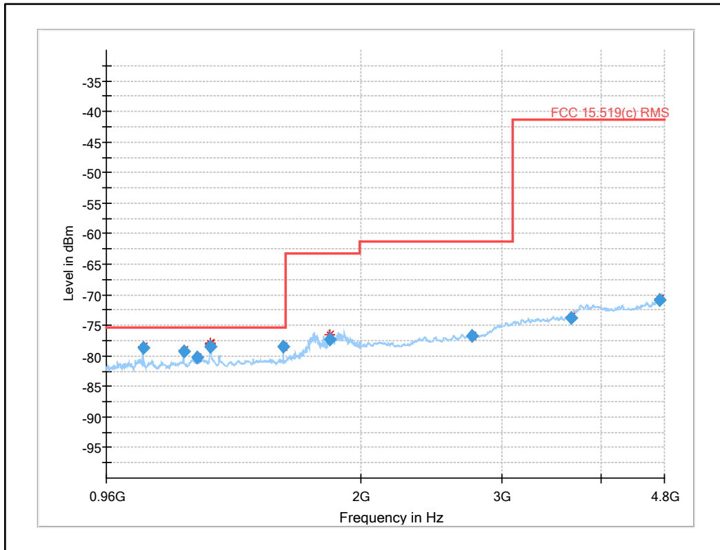
Plot 22: 960 MHz to 4.8 GHz (Limit acc. to §15.519 (c)), UWB test mode
