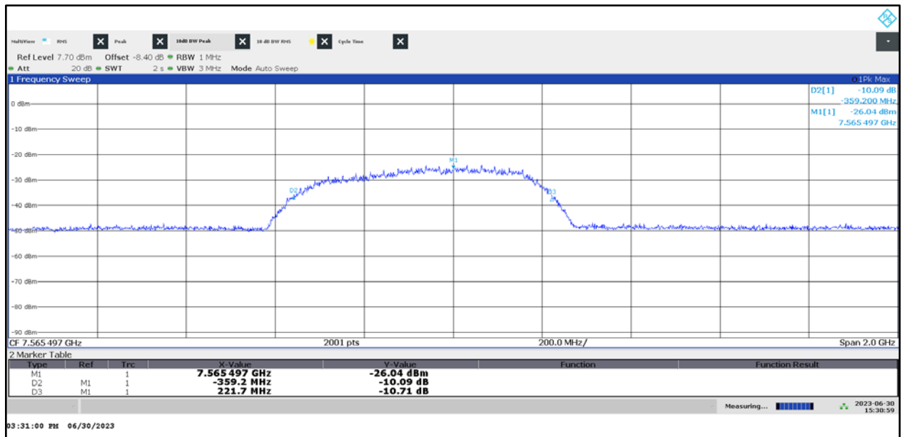
Plot 3: 10 dB bandwidth, UWB test mode channel 8
