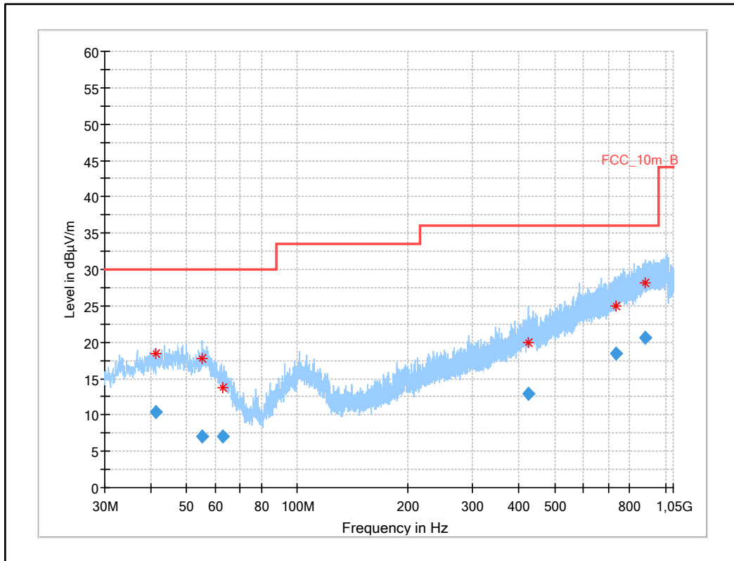
Plot 34: 30 MHz to 1 GHz, UWB test mode
