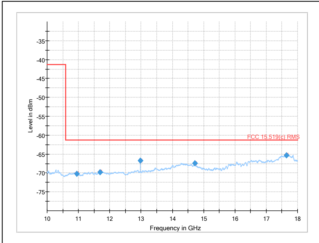
Plot 11: 10 GHz to 18 GHz, UWB test mode
