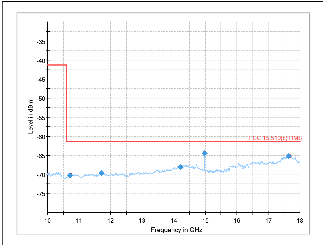
Plot 37: 10 GHz to 18 GHz, UWB test mode
