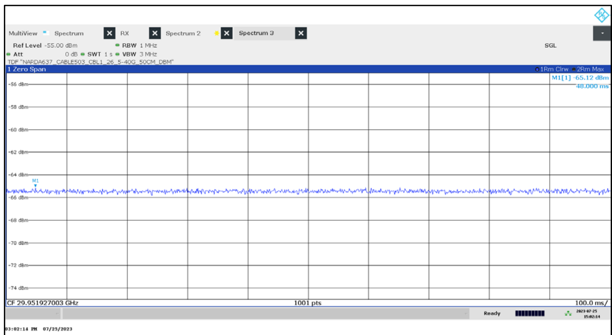
Plot 41: 29.9 GHz, UWB test mode zero span
