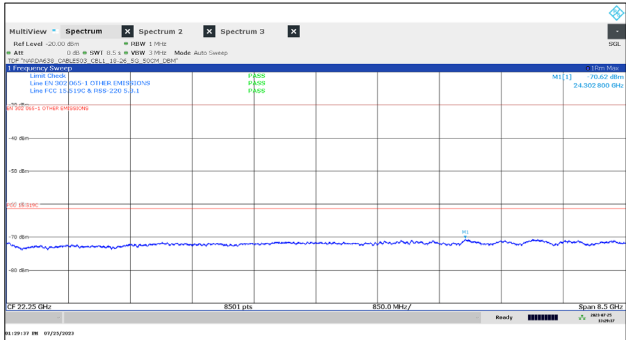
Plot 25: 18 GHz to 26.5 GHz, UWB test mode
