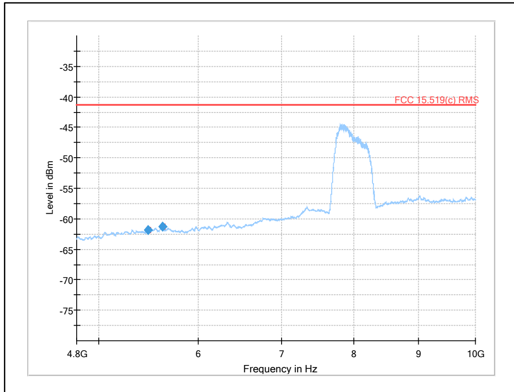
Plot 49: 4.8 GHz to 10 GHz, UWB test mode
