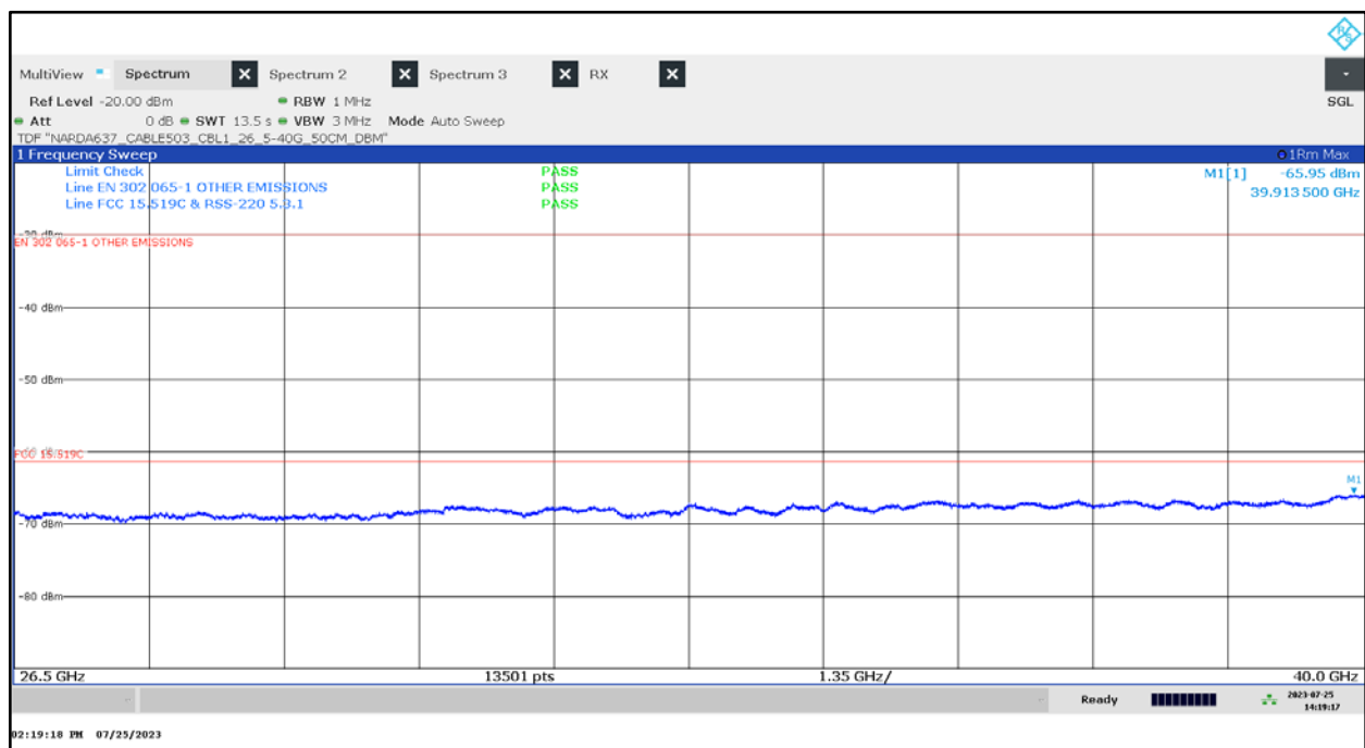
Plot 15: 26.5 GHz to 40.0 GHz, UWB test mode
