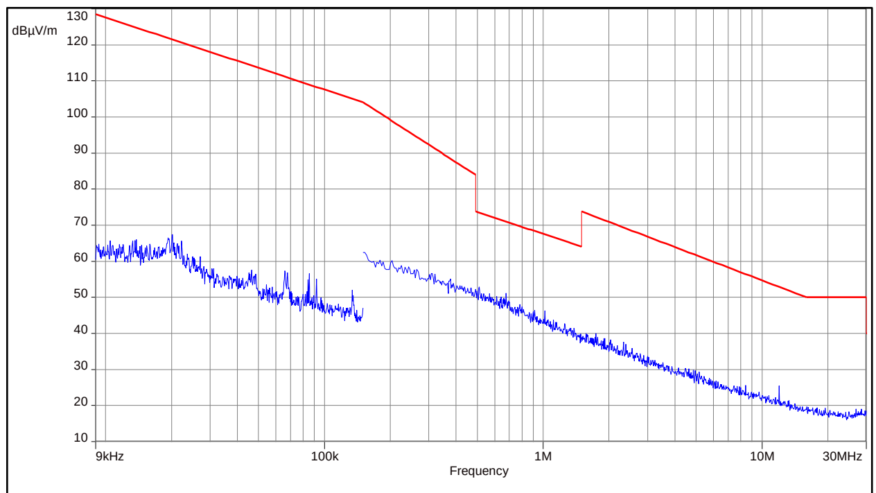
Plot 7: 9 kHz to 30 MHz, UWB test mode
