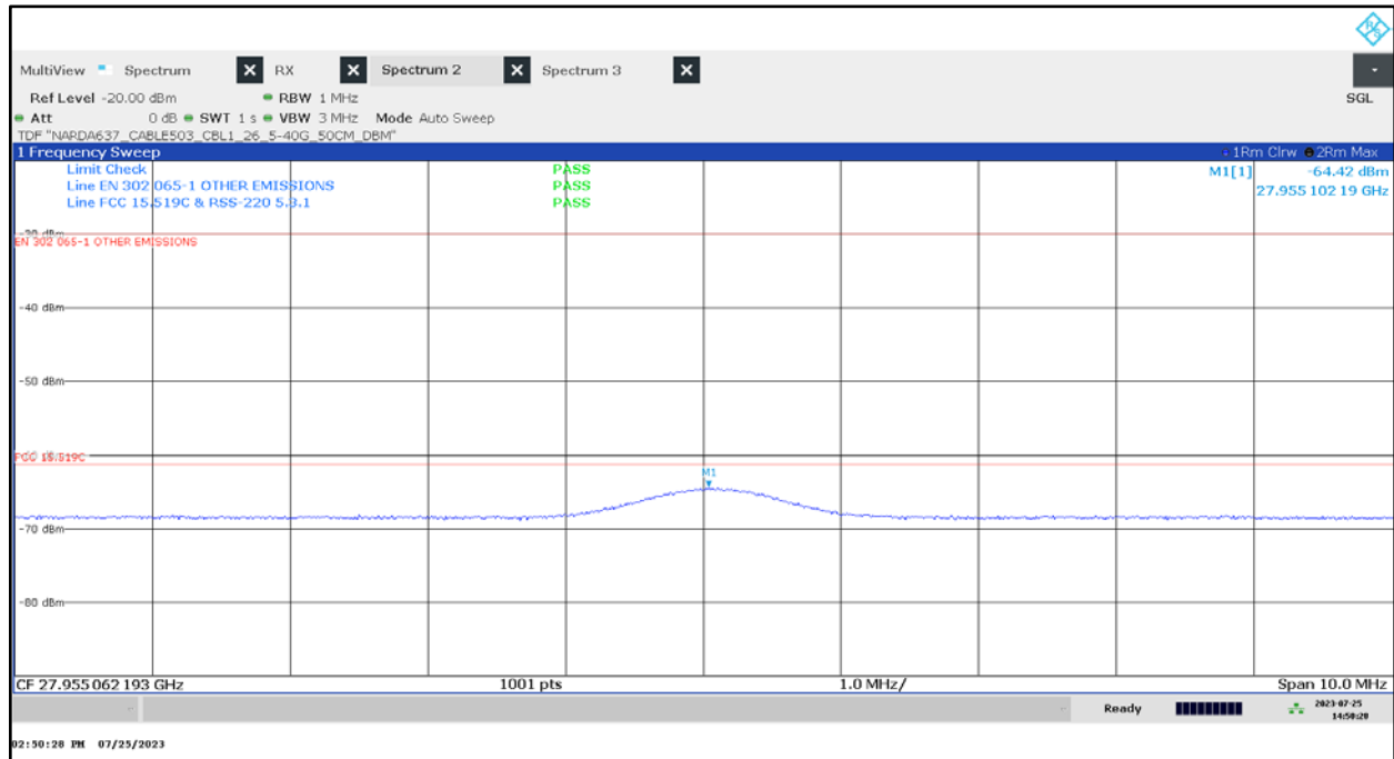
Plot 27: 27.9 GHz, UWB test mode 10 MHz span
