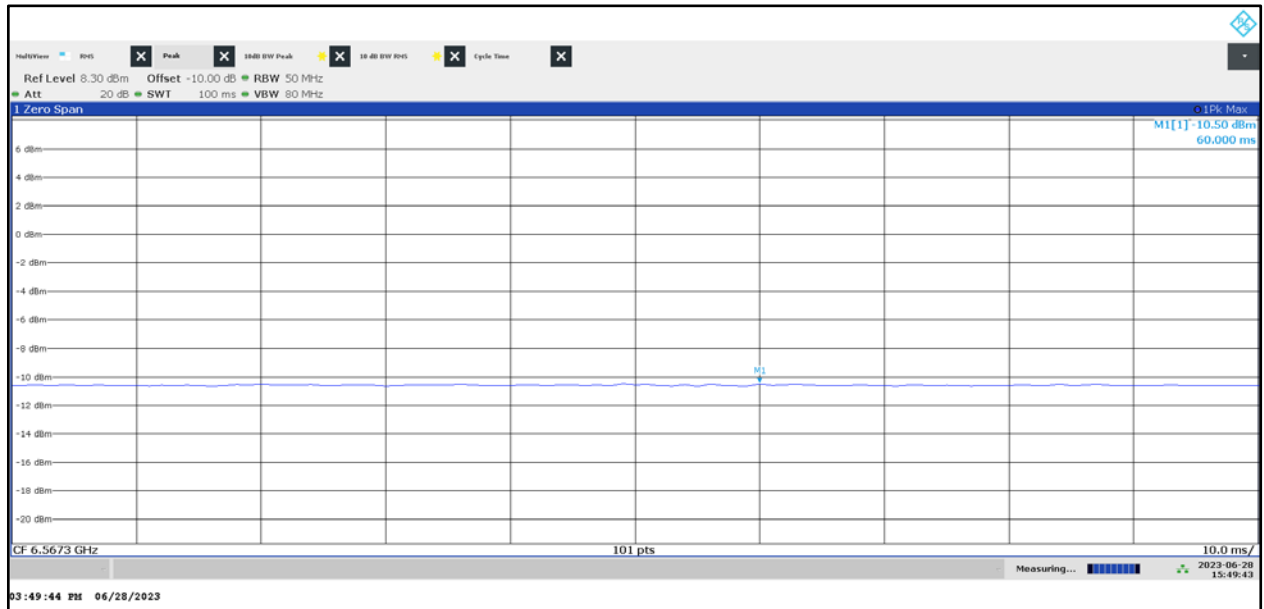
Plot 6: Fundamental emission (UWB test mode): Max Peak
