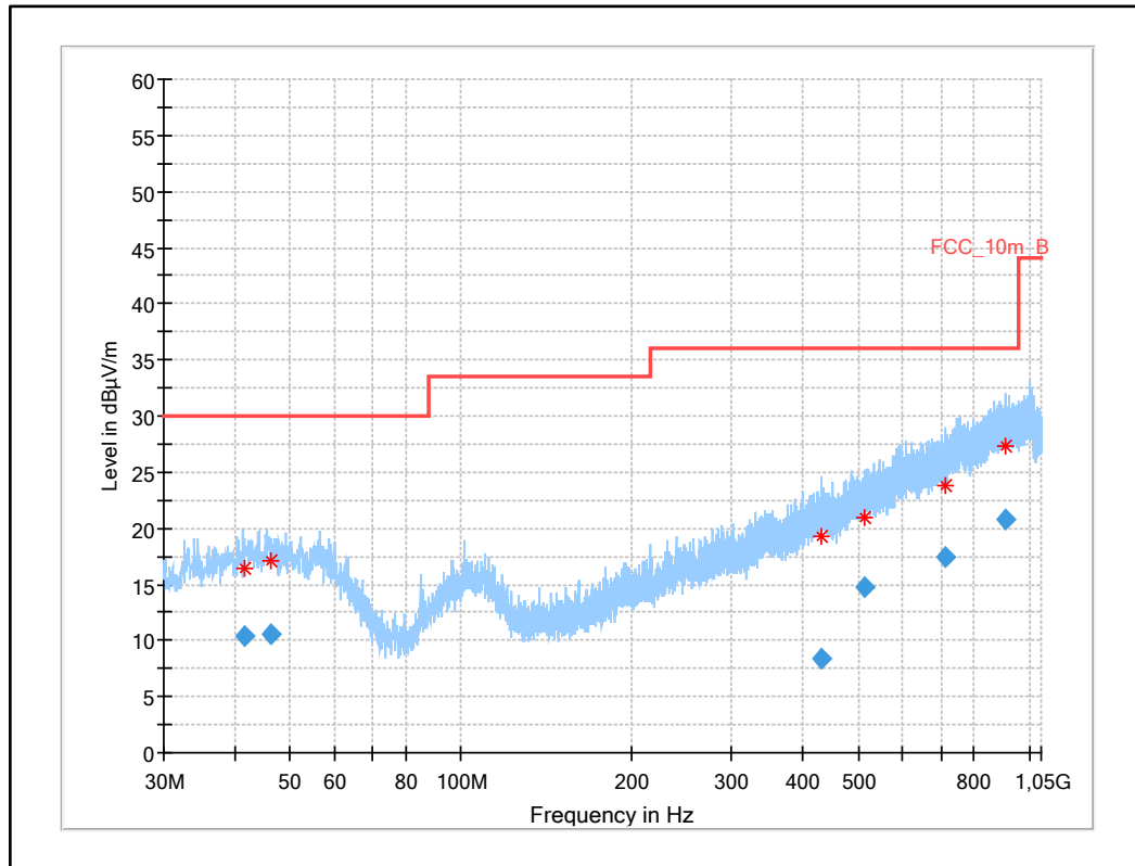
Plot 8: 30 MHz to 1 GHz, UWB test mode
