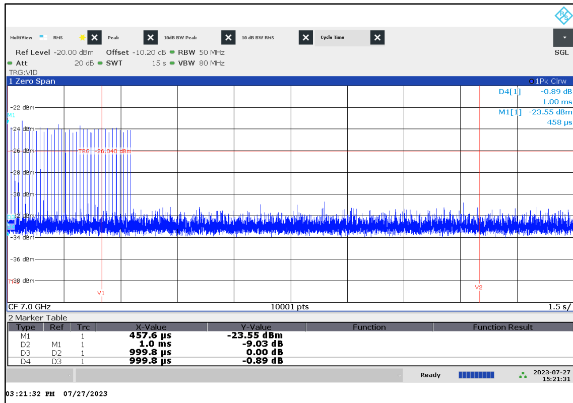
Plot 58: Emissions of the EUT, only at the beginning with associated receiver (Normal mode CH6)
