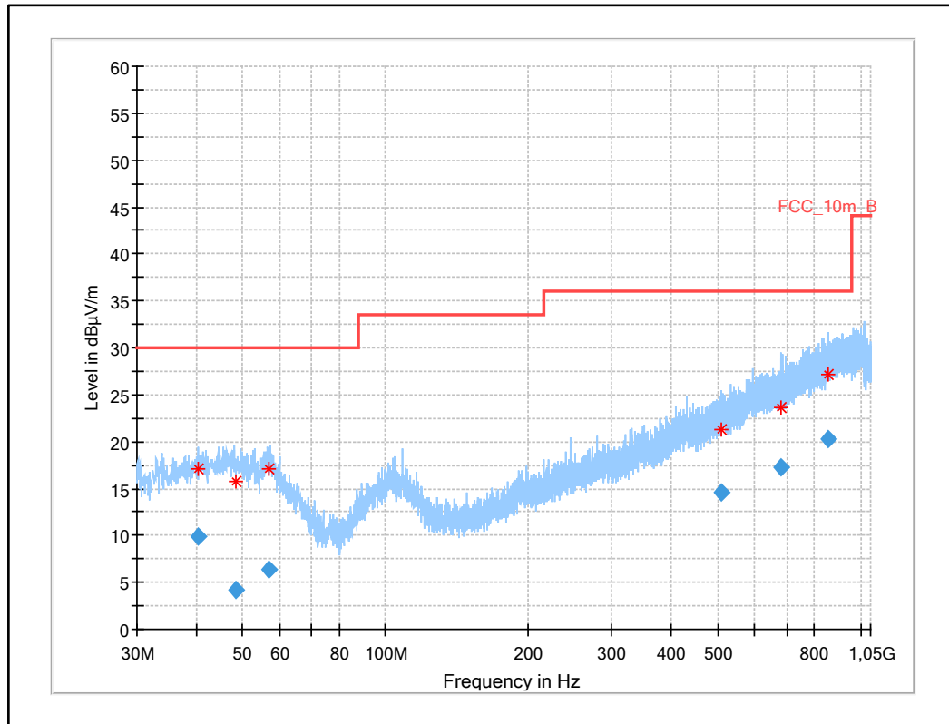
Plot 21: 30 MHz to 1 GHz, UWB test mode
