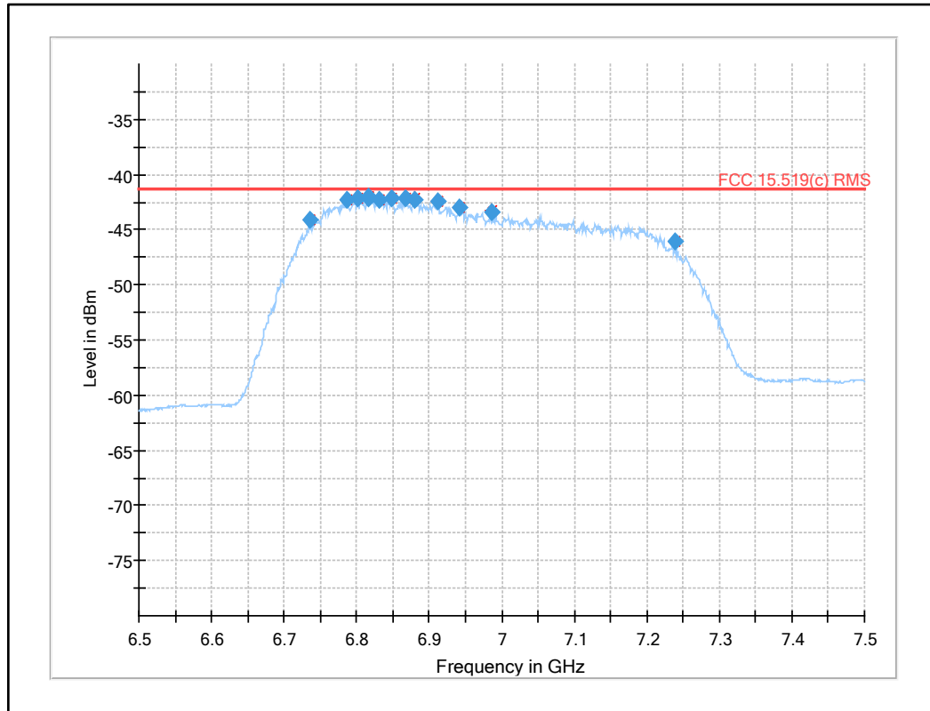
Plot 18: Fundamental emission (UWB test mode): RMS
