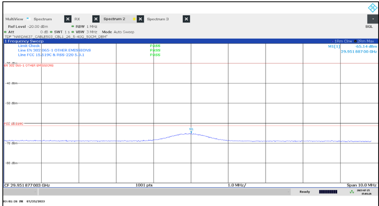
Plot 40: 29.9 GHz, UWB test mode 10 MHz span
