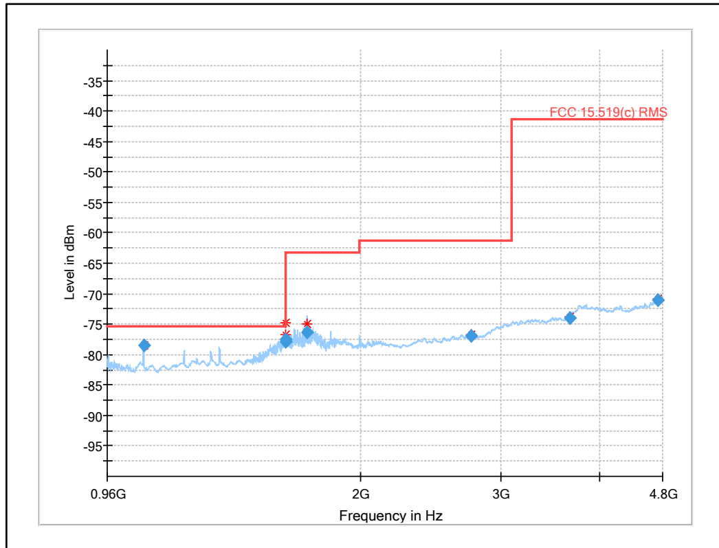
Plot 48: 960 MHz to 4.8 GHz (Limit acc. to §15.519 (c)), UWB test mode
