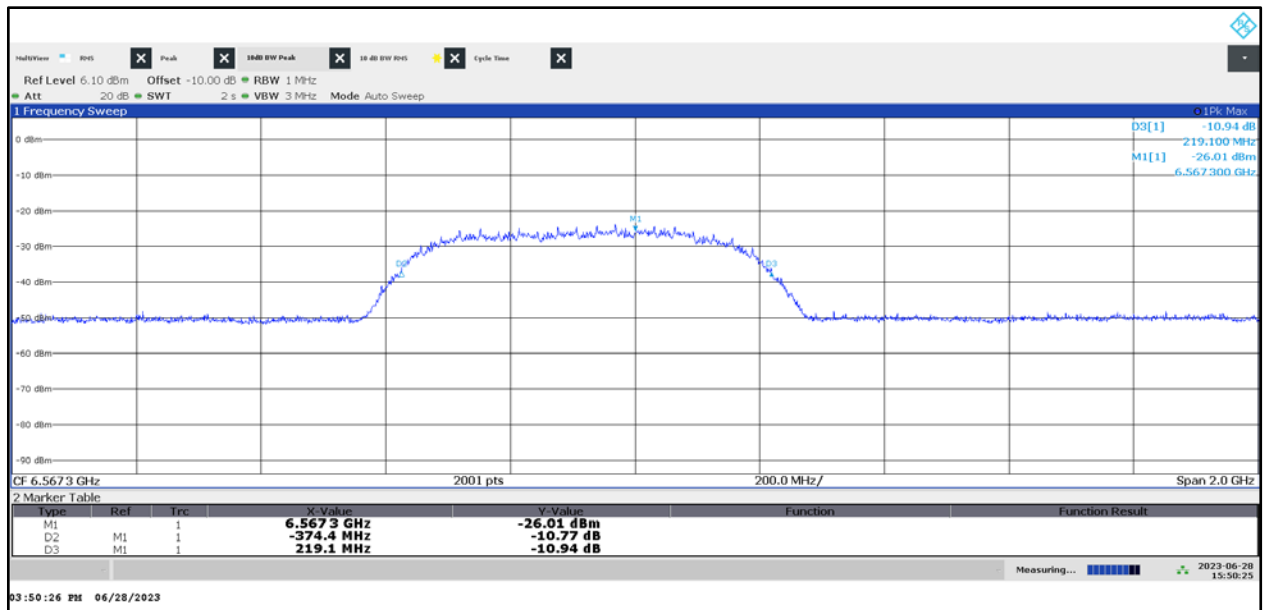
Plot 1: 10 dB bandwidth, UWB test mode channel 5
