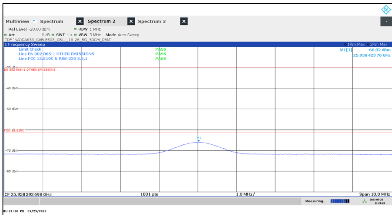
Plot 13: 25.9 GHz, UWB test mode 10MHz span
