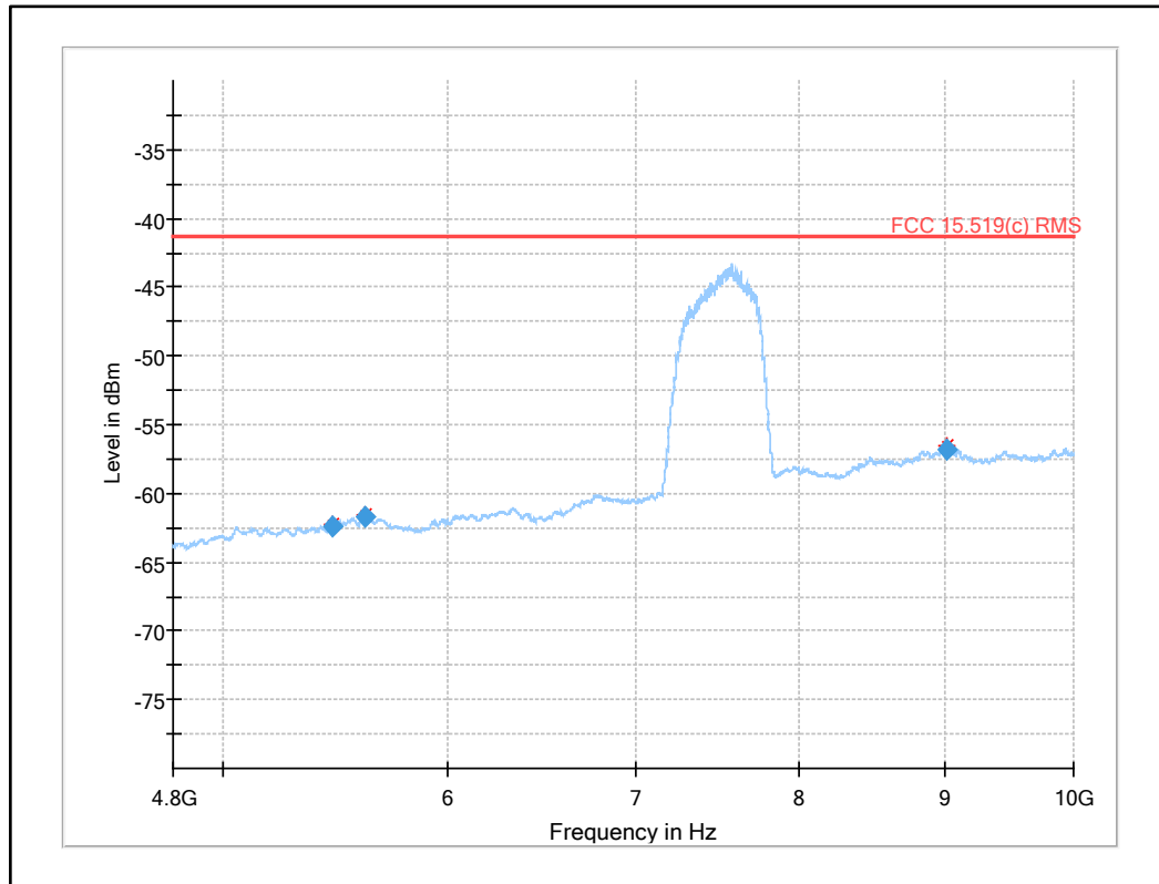
Plot 36: 4.8 GHz to 10 GHz, UWB test mode
