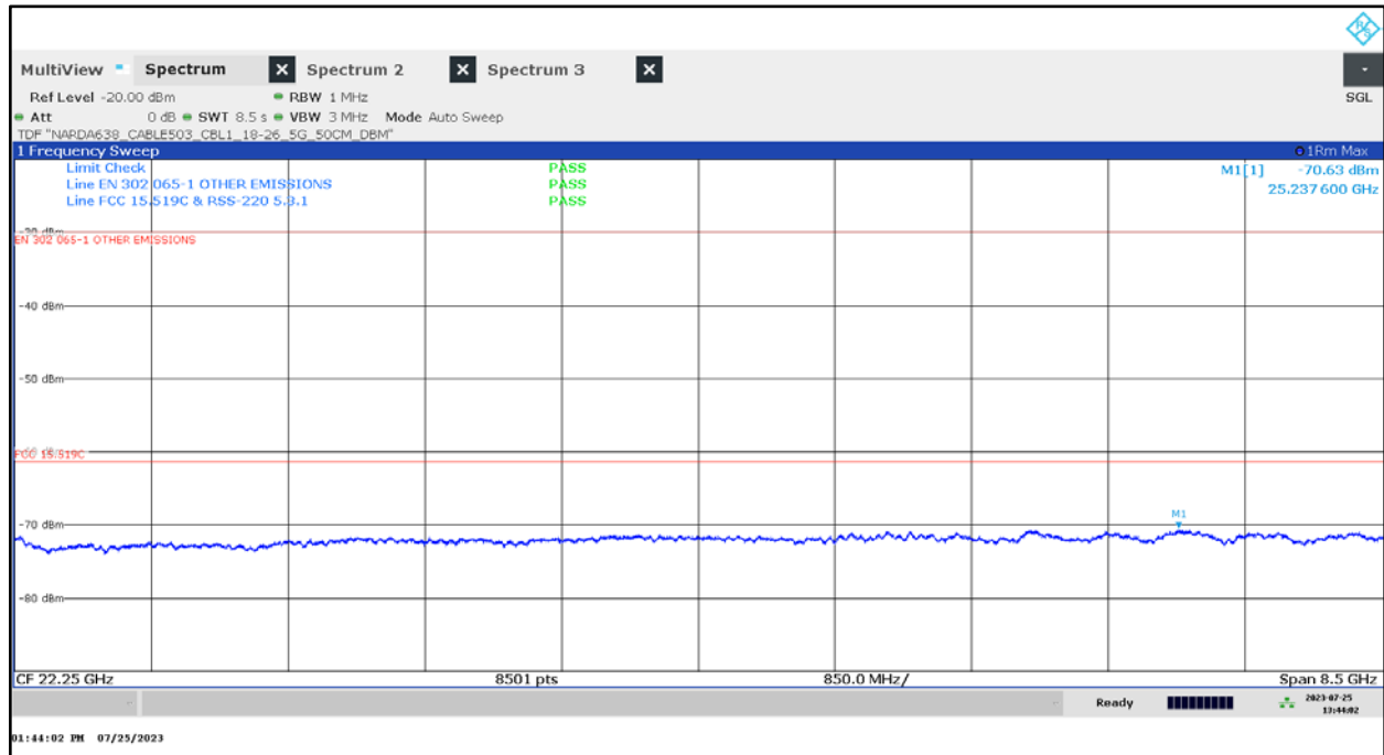
Plot 38: 18 GHz to 26.5 GHz, UWB test mode
