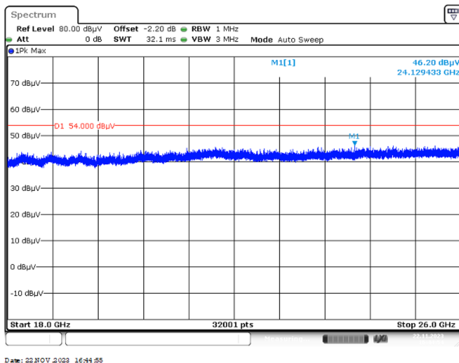
Plot 8: 18 GHz to 26 GHz, TX mode, vertical & horizontal polarization, 2 Msps, valid for all channels
