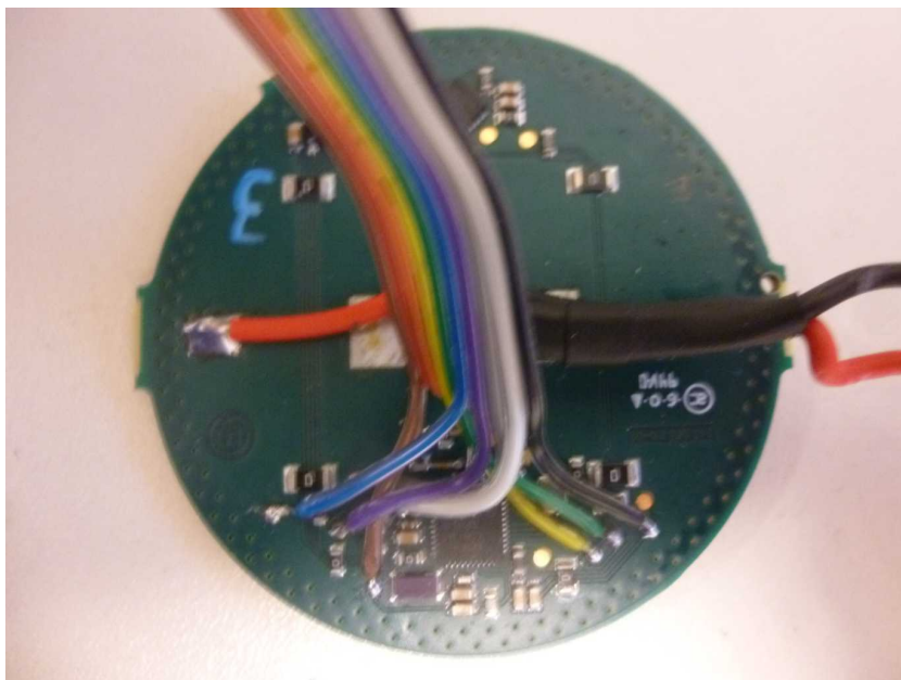
Photo 8: PCB front side view
