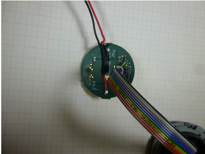
Photo 9: PCB front side view
