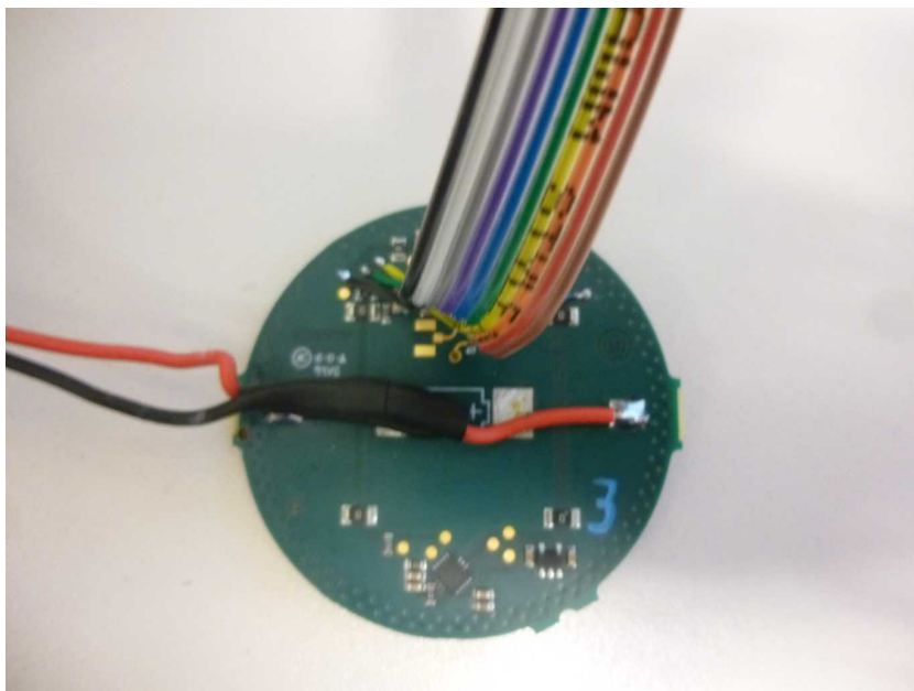
Photo 6: PCB front side view
