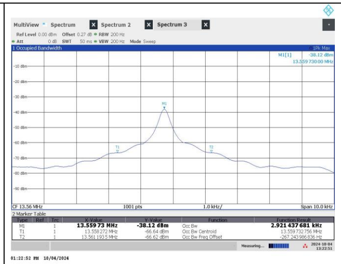
99 % Bandwidth
