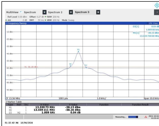
20 dB Bandwidth
