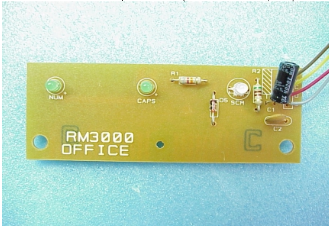
Figure 11 M/N OFFICE 300, Internal View (LED / Control Board, Component Side)
