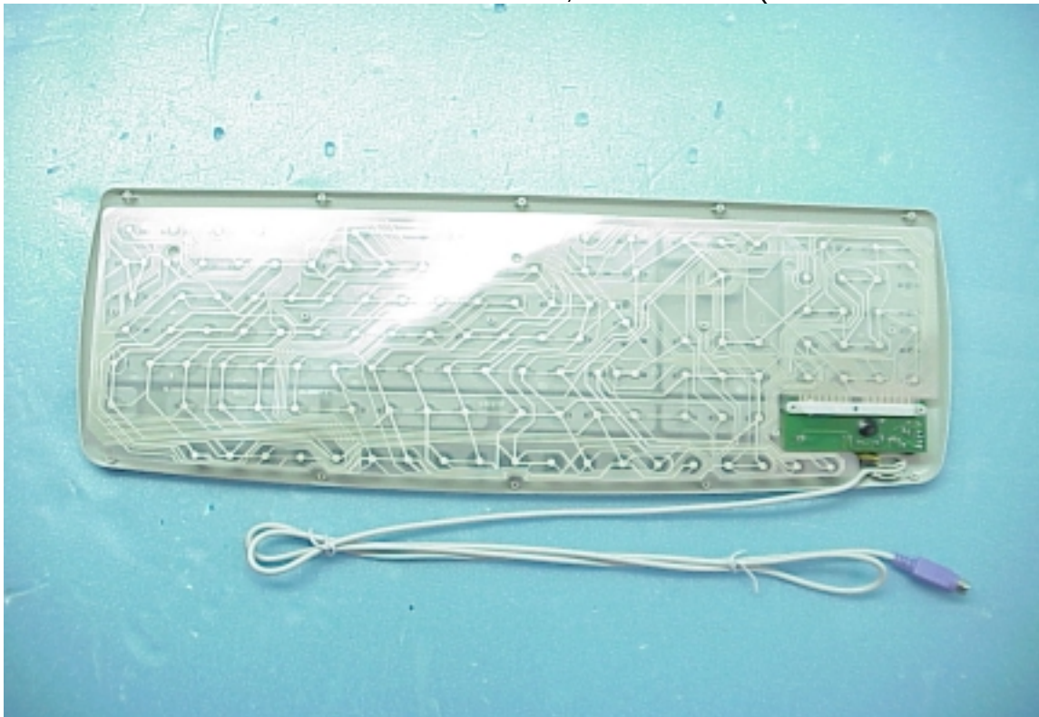
Figure 10 M/N OFFICE 300, Internal View (Removed Bottom Cover)
