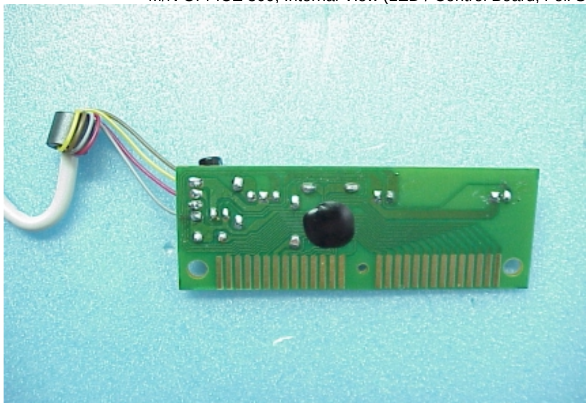
Figure 12 M/N OFFICE 300, Internal View (LED / Control Board, Foil Side)
