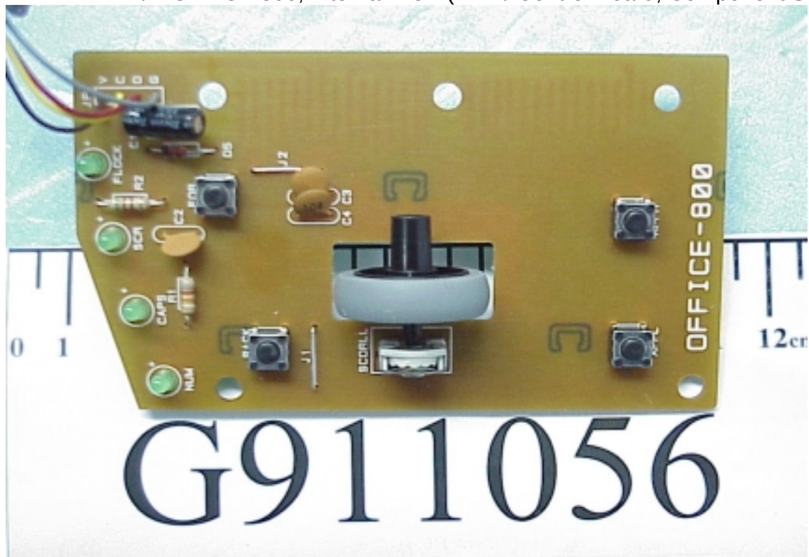
Figure 6 M/N OFFICE 800, Internal View (LED / Control Board, Foil Side)
