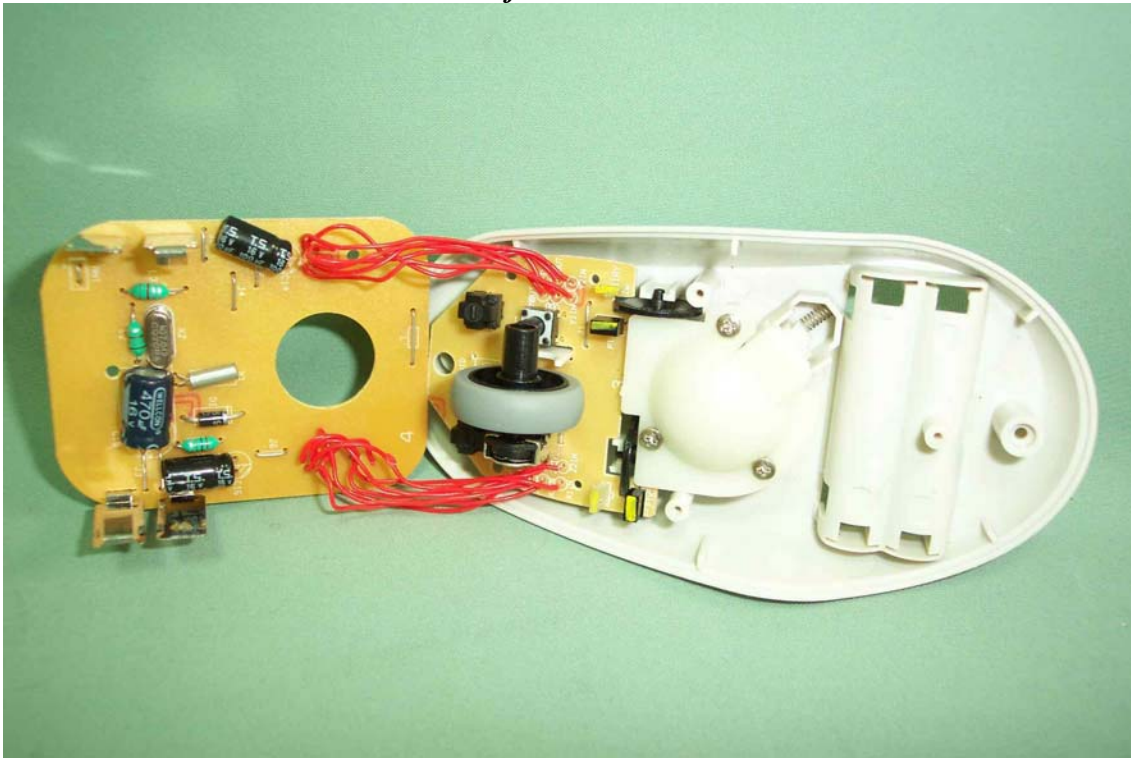
Internal of ACE-800BW --- 3
