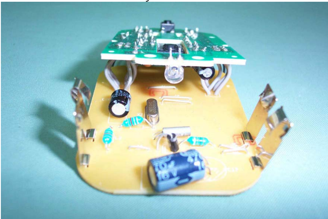
Internal of ACE-800AW --- 6
