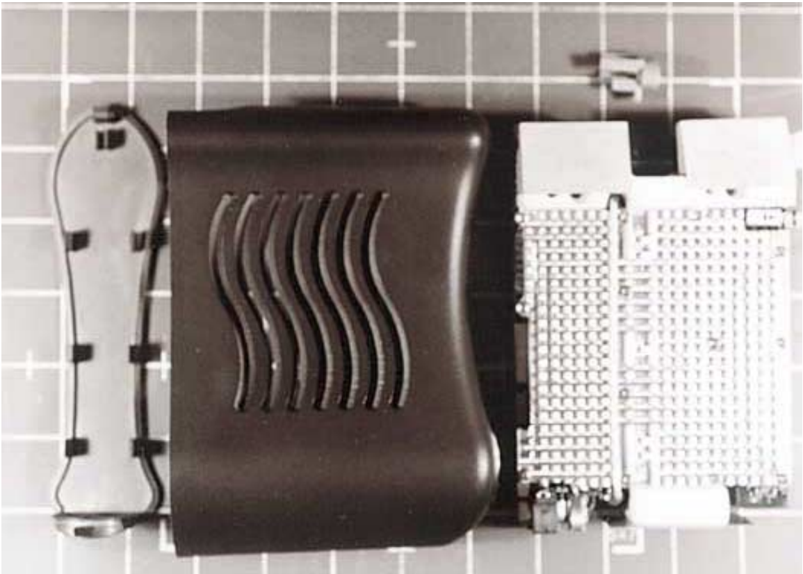
PCB Assembly Removed from Enclosure
