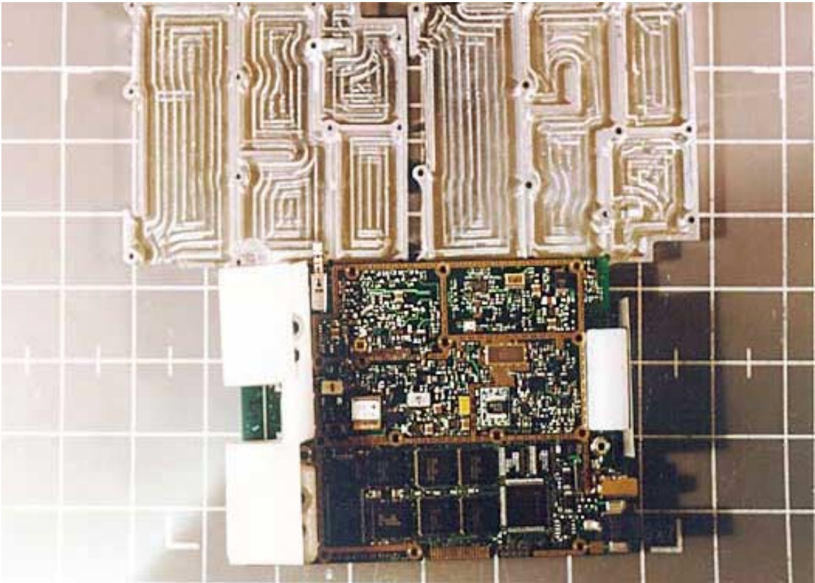
Shields Removed from PCB Assembly
