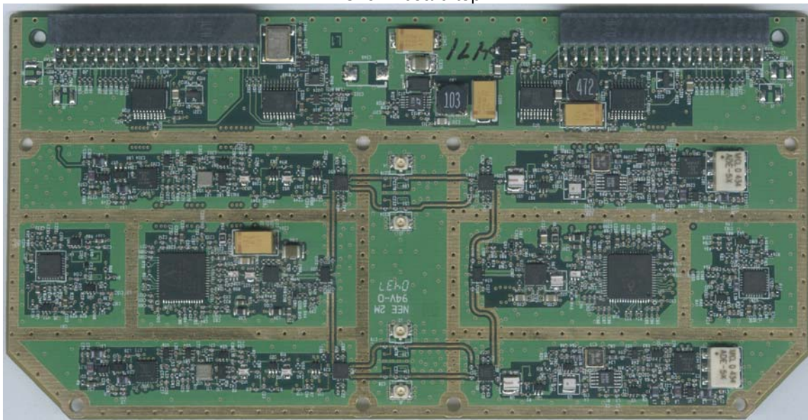
132621 board top
