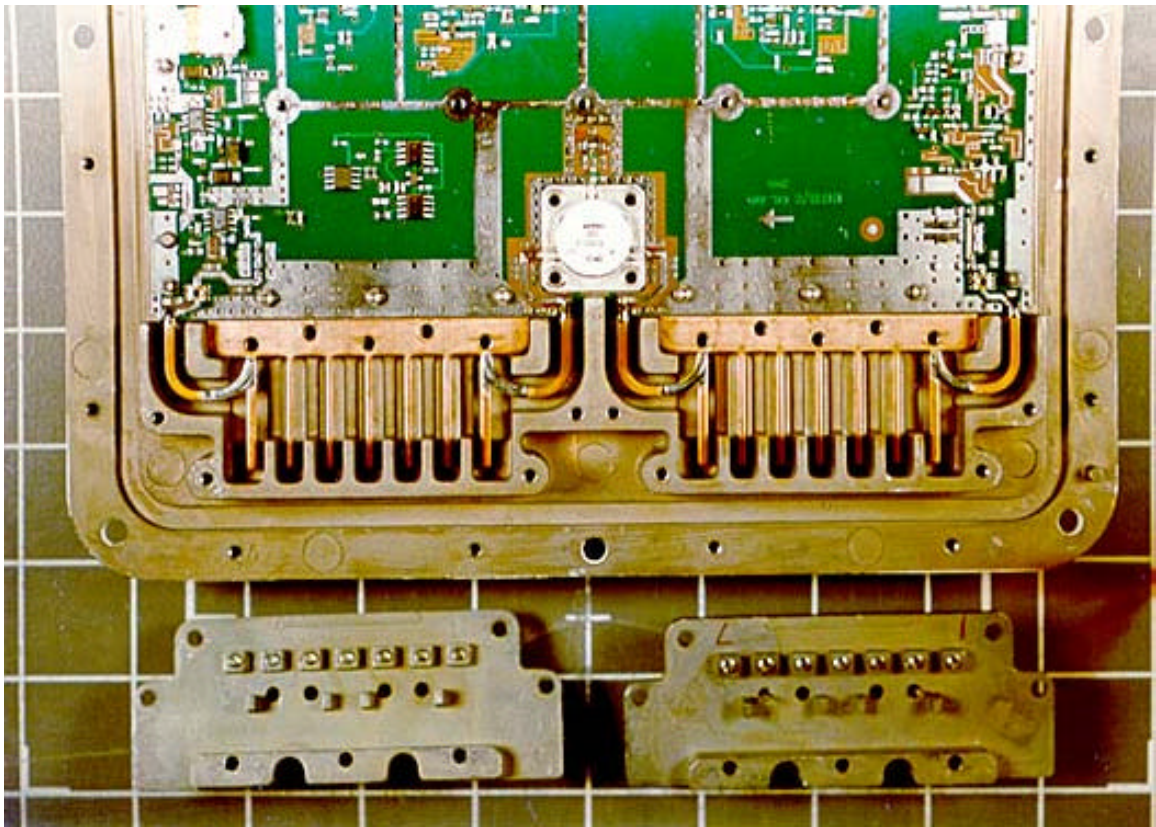
Inside Back Close-up of Tuner Portion
