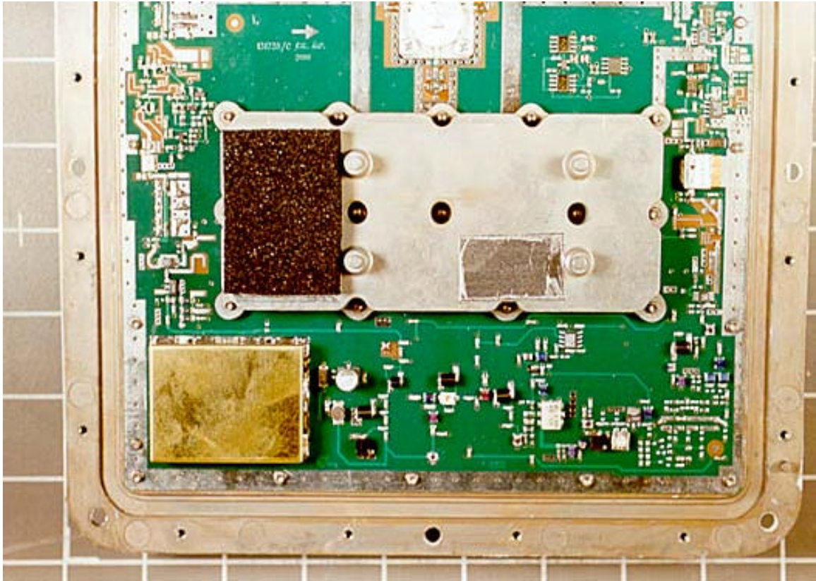
Inside Back Close-up of Right Side
