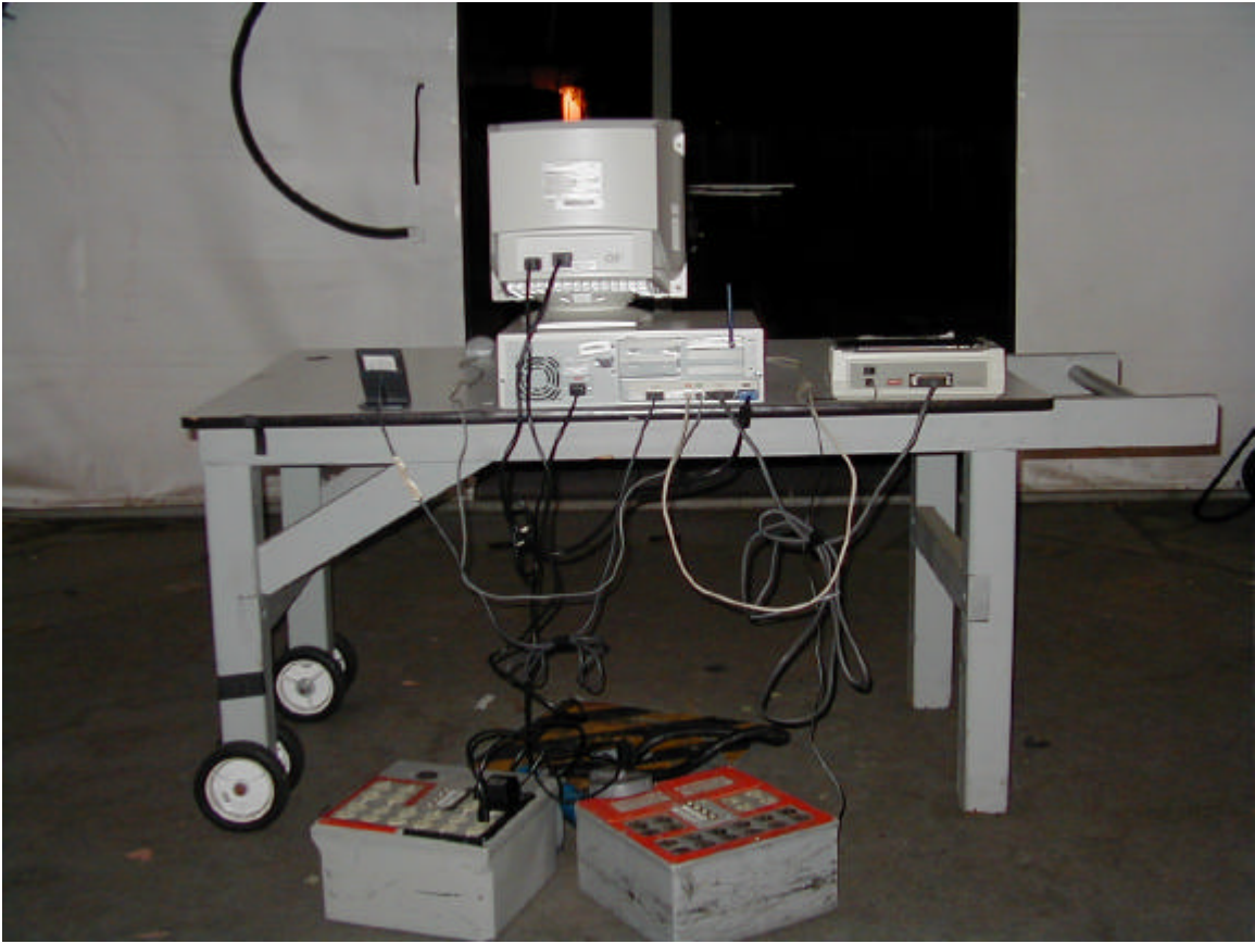
Radiate emission above 1 GHz.
