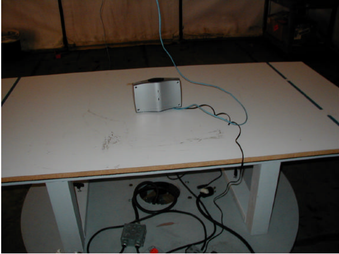
Above 1 GHz Test Setup Photo (Back Side)
