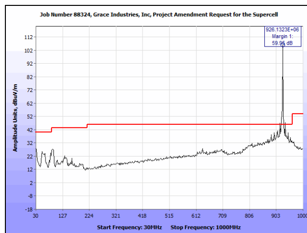
Plot 15. Radiated Spurious Emissions, 30 MHz – 1 GHz, High Channel
