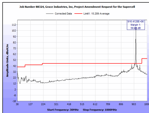
Plot 14. Radiated Spurious Emissions, 30 MHz – 1 GHz, Mid Channel
