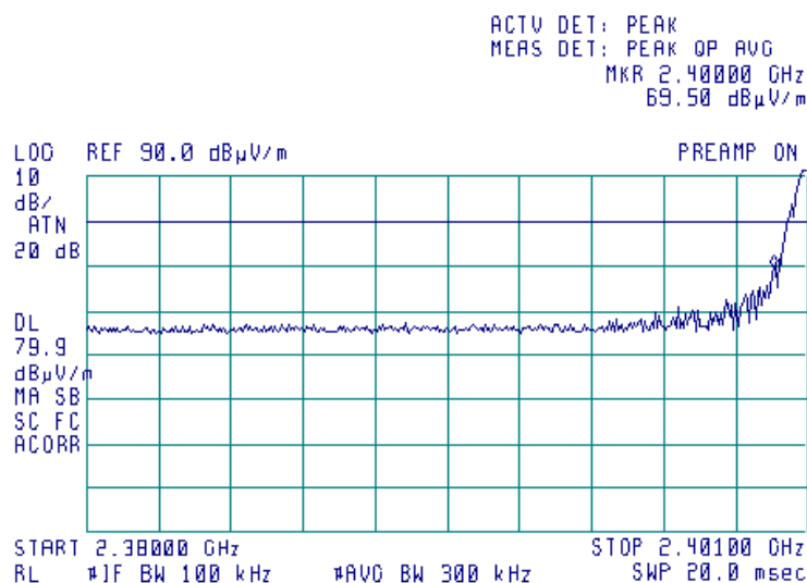
Plot 7.7.7 The highest band edge emission at low carrier frequency with hopping function enabled, Restricted Band
