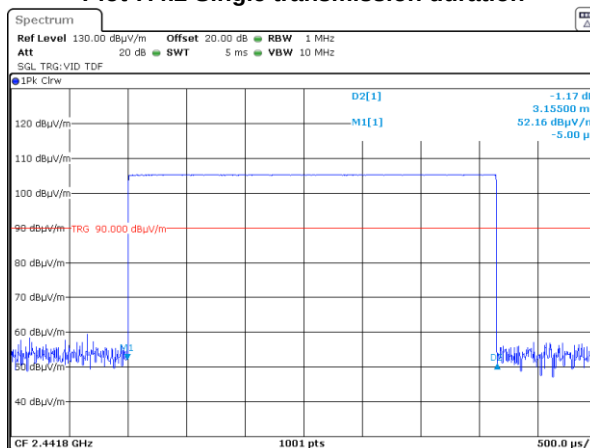
Plot 7.4.2 Single transmission duration
