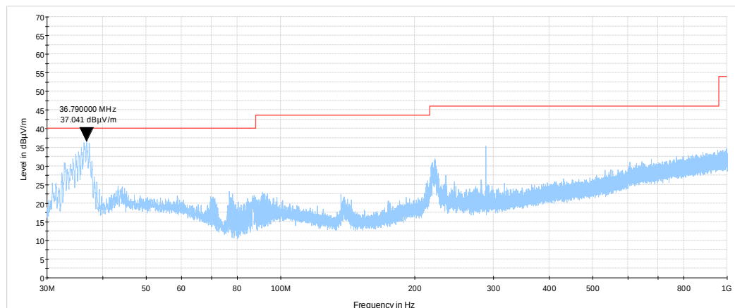
Plot 7.6.9 Radiated emission measurements from 30 to 1000 MHz at the high carrier frequency
