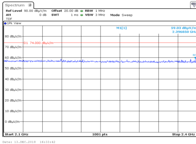
Plot 7.6.16 Radiated emission measurements from 2100 to 2400 MHz at the high carrier frequency
