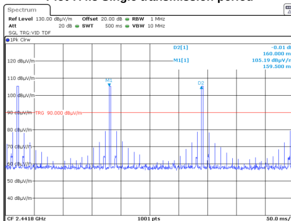
Plot 7.4.3 Single transmission period
