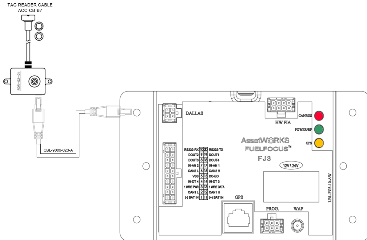
Figure 13: Connecting the Driver ID reader to the FJ3
