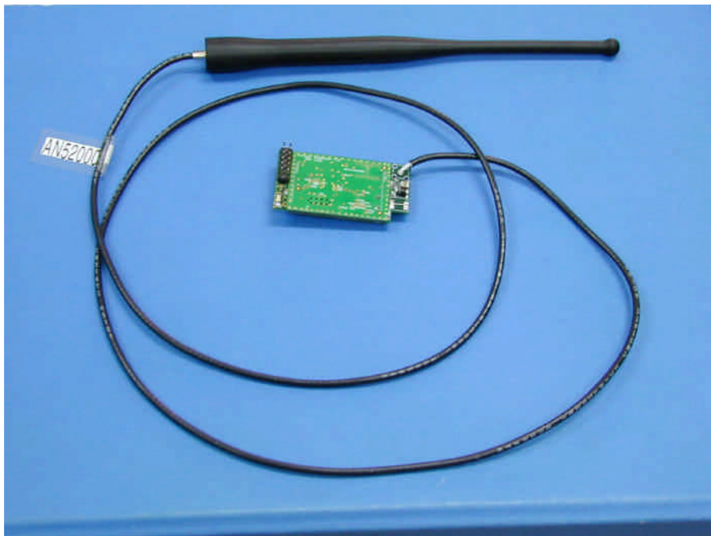
Transceiver module, view with antenna
