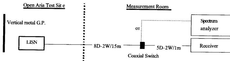
Cables for Conducted emission Test
