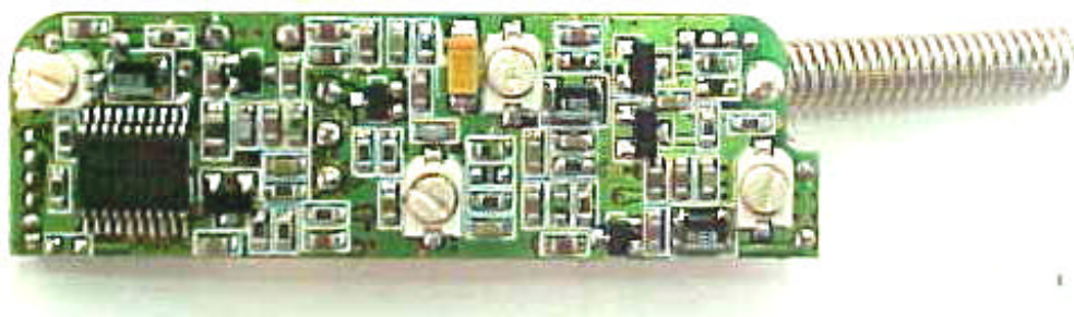
Internal PCB # 1 – Component Side
