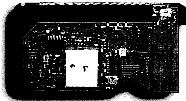
MODEL CP-AV03 L BAND RX SIDE 1
