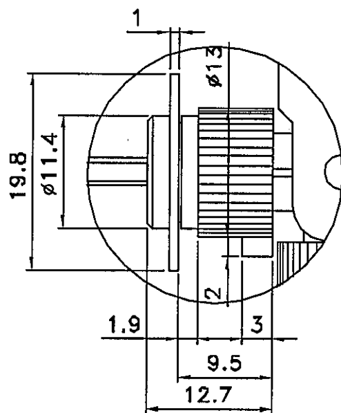
Detail 'Y' 3:1 TOLERANCES: \pm 0.1
