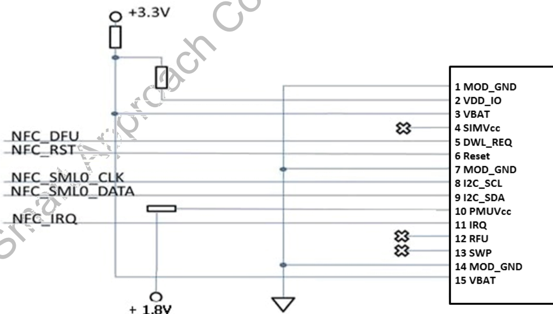
Figure 7 Main Board Design W/O UICC Reference
