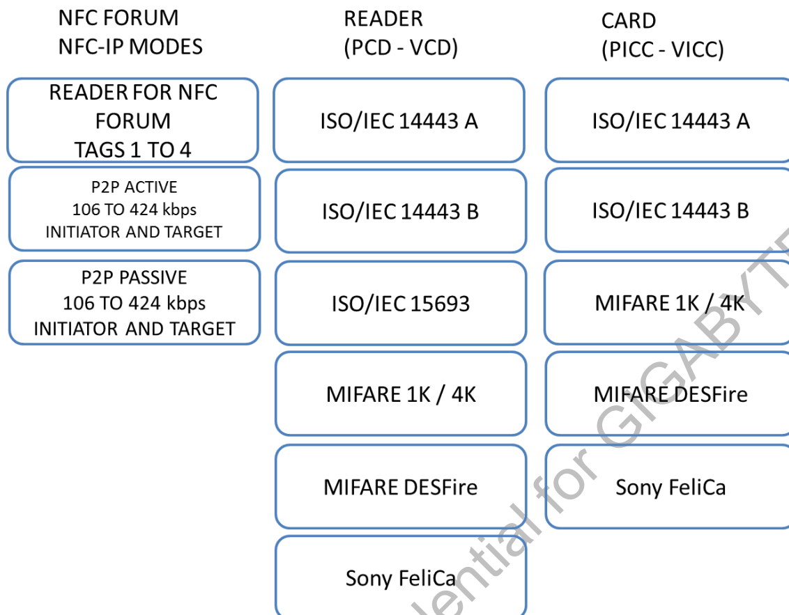
Figure 4 Transmission Modes
