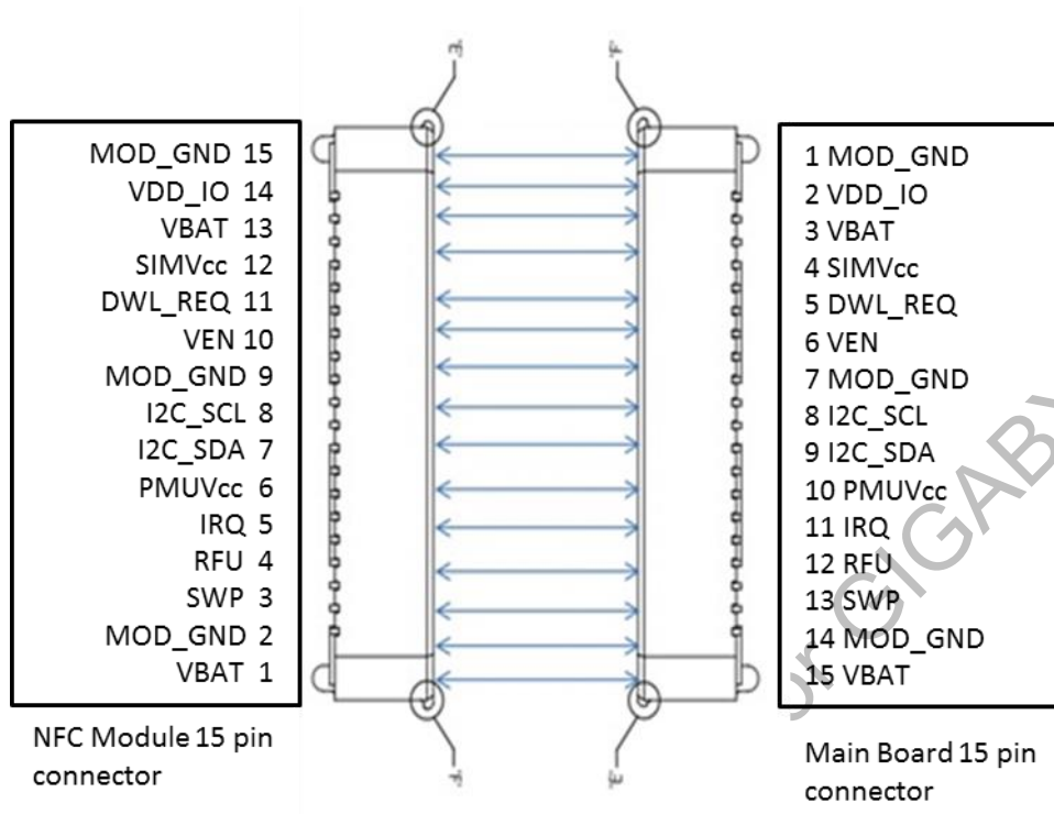
Figure 6 Connection Recommendation
