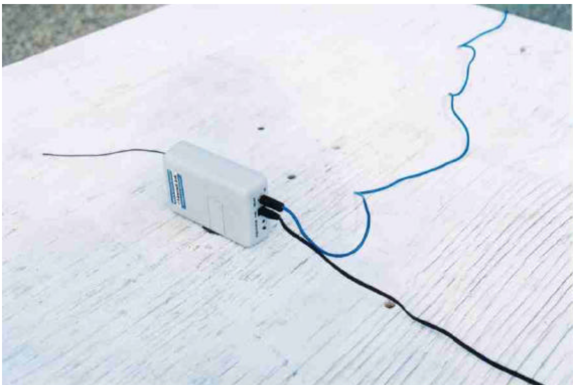
Figure 2. DUT
