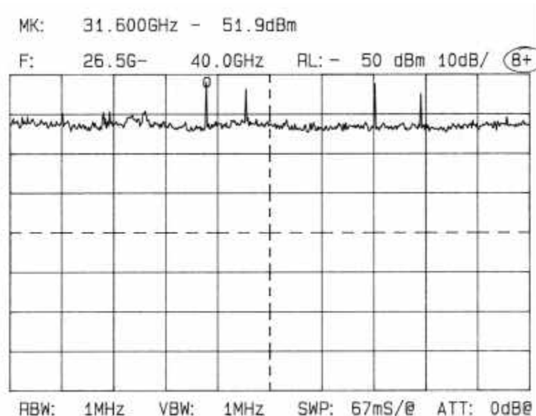
Plot 4.1.21 Out of band emission measurements with Agilis module
