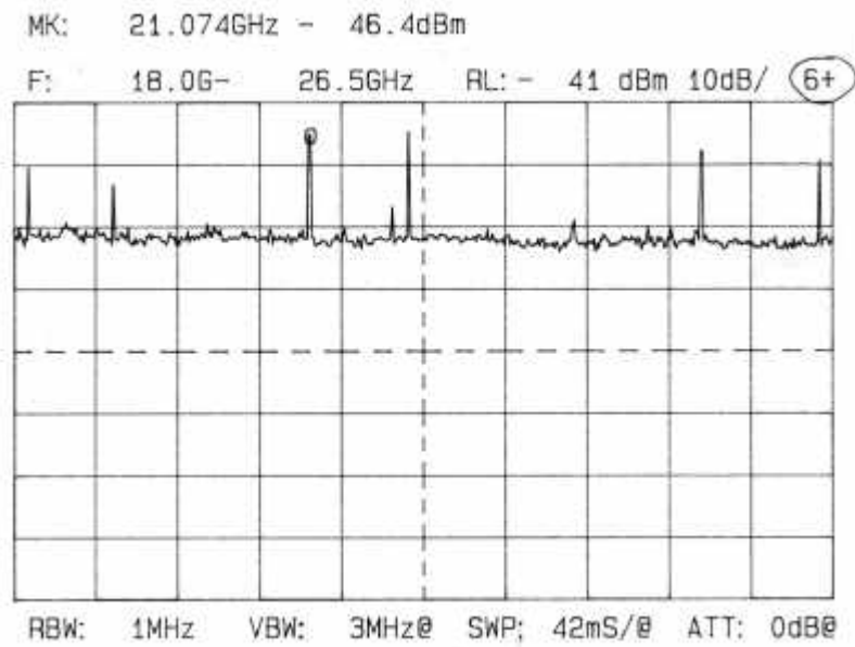
Plot 4.1.7 Out of band emission measurements with Microwave Solutions module
