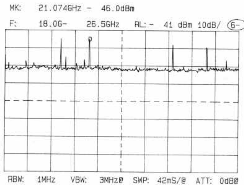
Plot 4.1.8 Out of band emission measurements with Microwave Solutions module
