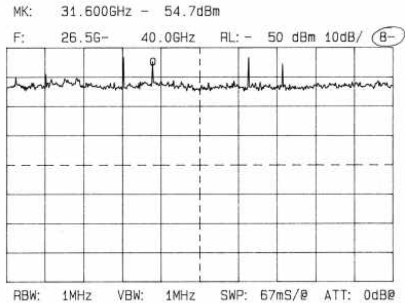
Plot 4.1.20 Out of band emission measurements with Agilis module
