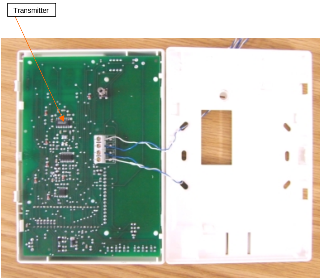
Photograph No.2 RP128KCLP keypad internal view
