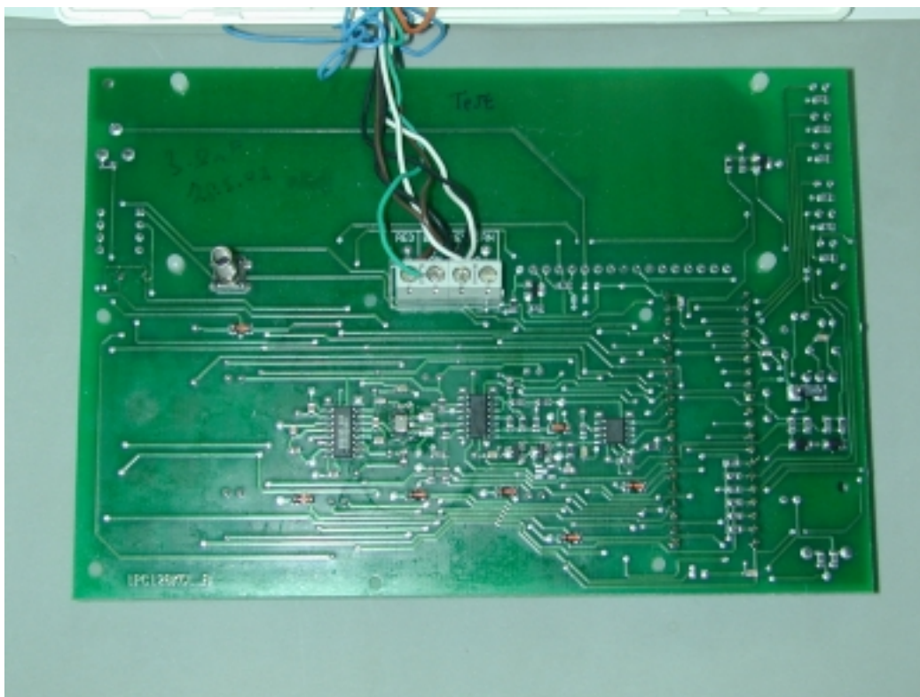
Photograph No.4 RP128KCLP keypad PCB second side view
