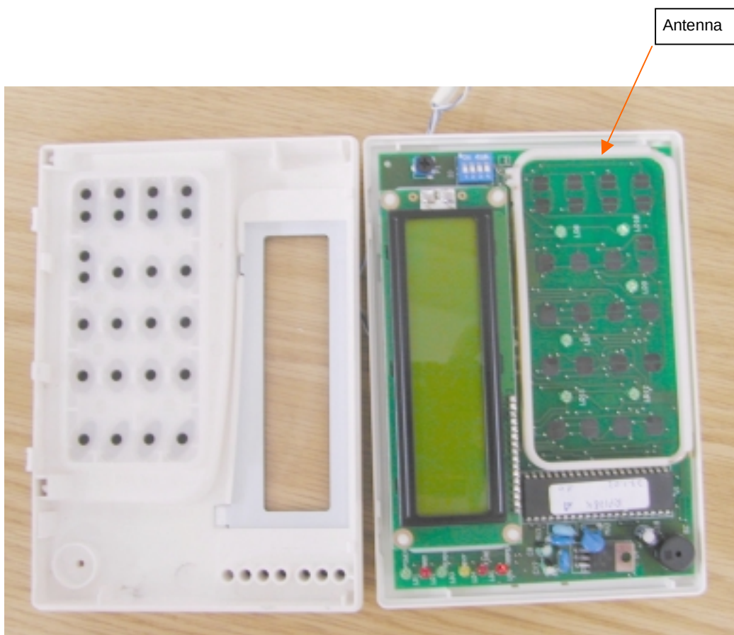
Photograph No.1 RP128KCLP keypad internal view
