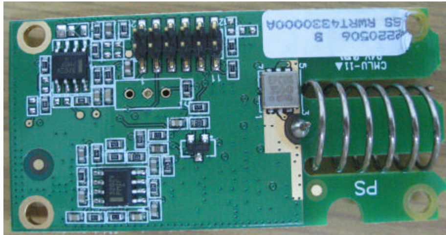
Photograph No.7 Print side of the RF PCB
