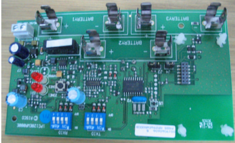
Photograph No.4 Main PCB without RF PCB, component side
