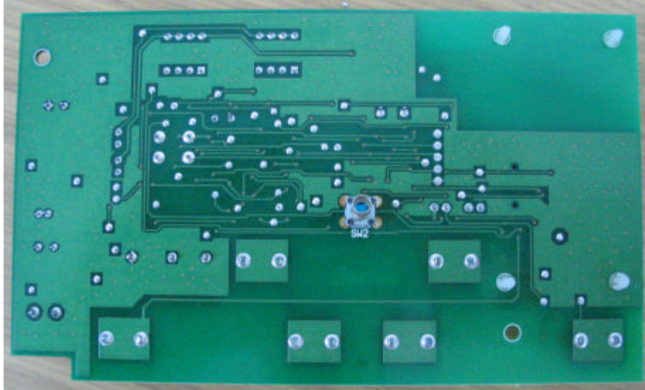
Photograph No.5 Main PCB, printside
