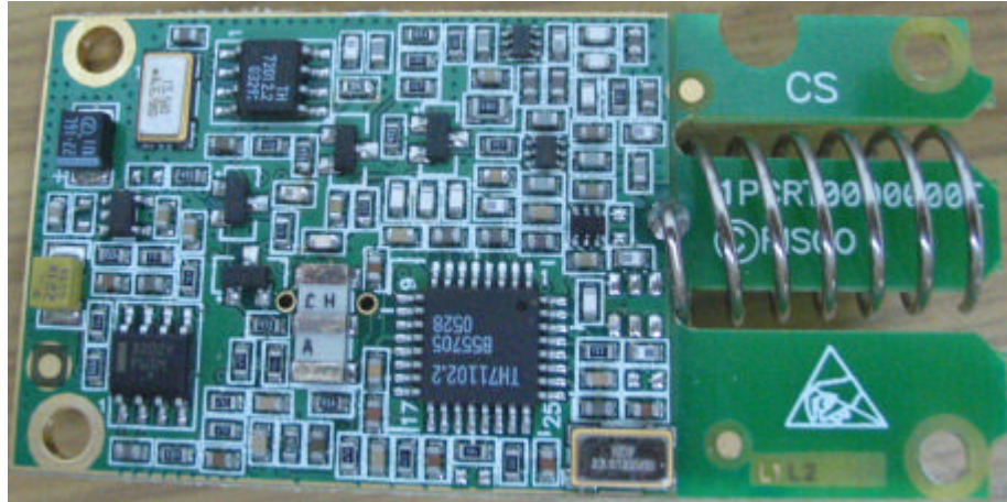
Photograph No.6 Component side of the RF PCB
