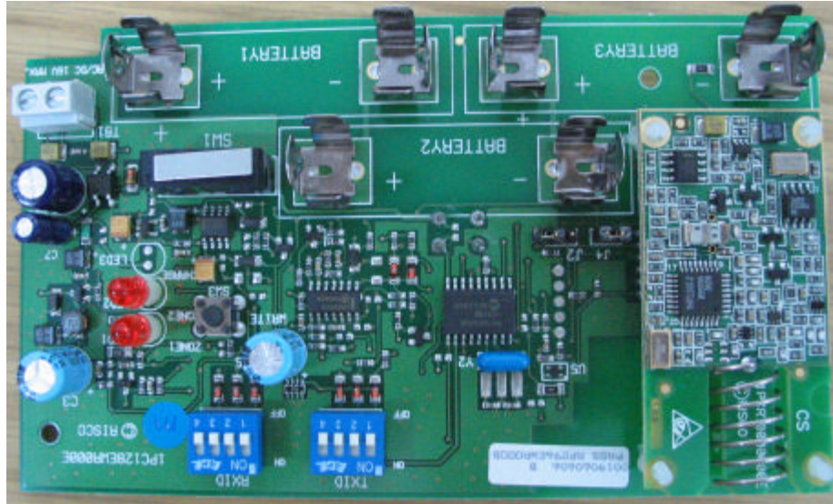
Photograph No.3 Main and RF PCBs, component side
