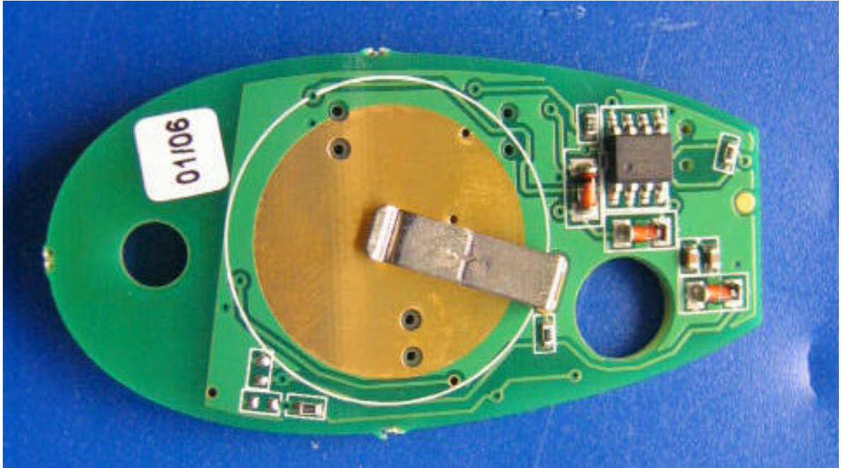
Photograph No.3 Print side of the main/RF PCB
