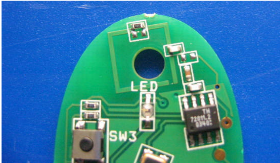
Photograph No.4 Antenna assembly
