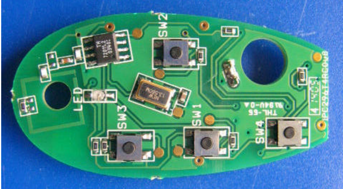
Photograph No2 Component side of the main/RF PCB
