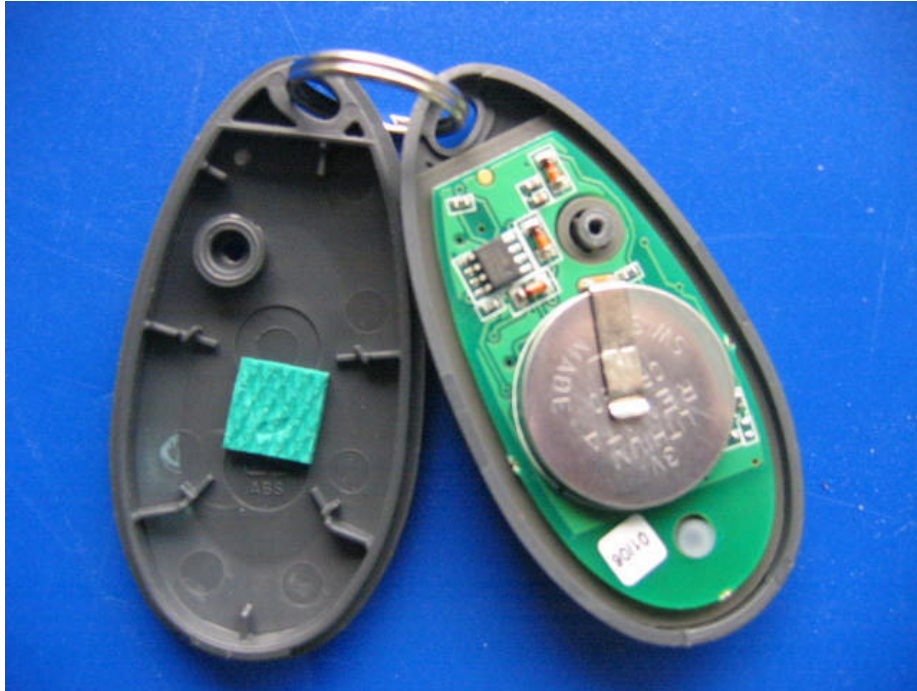
Photograph No.1 RP296T4RC00A transmitter internal view
