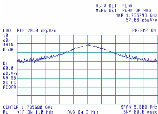
Plot 7.2.13 Radiated emission measurements at the forth harmonic frequency
