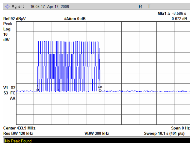
Plot 7.2.26 Transmission train duration
