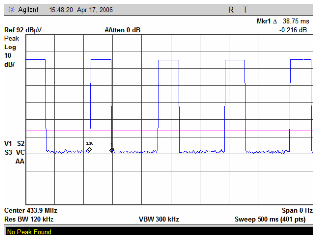
Plot 7.2.25 Transmission burst period
