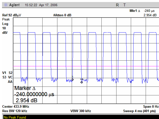
Plot 7.2.23 Transmission pulse period
