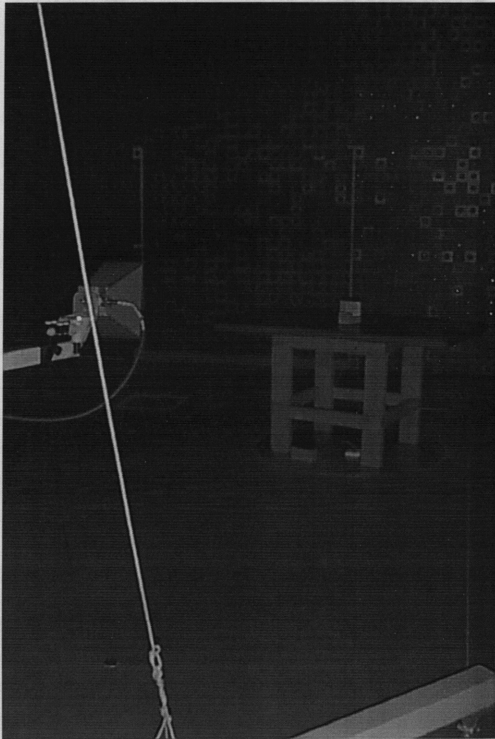
Radiated Emission Measurements Setup Photograph 3.1.3
