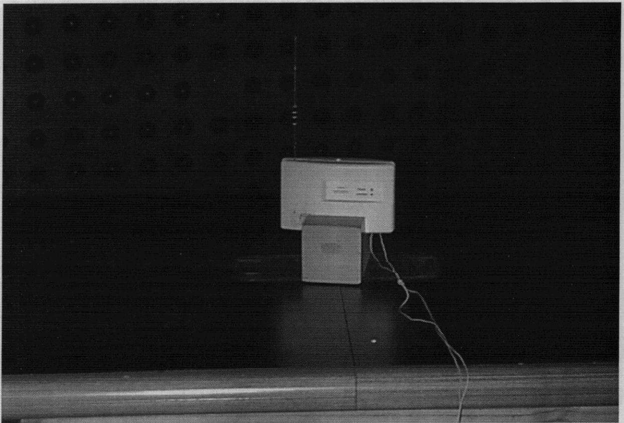
Radiated Emission Measurements Setup Photograph 3.1.2
