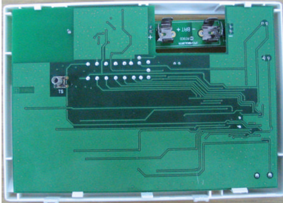
Photograph No.5 Main and RF PCB, second side
