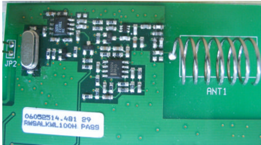
Photograph No.6 Component side of the RF PCB
