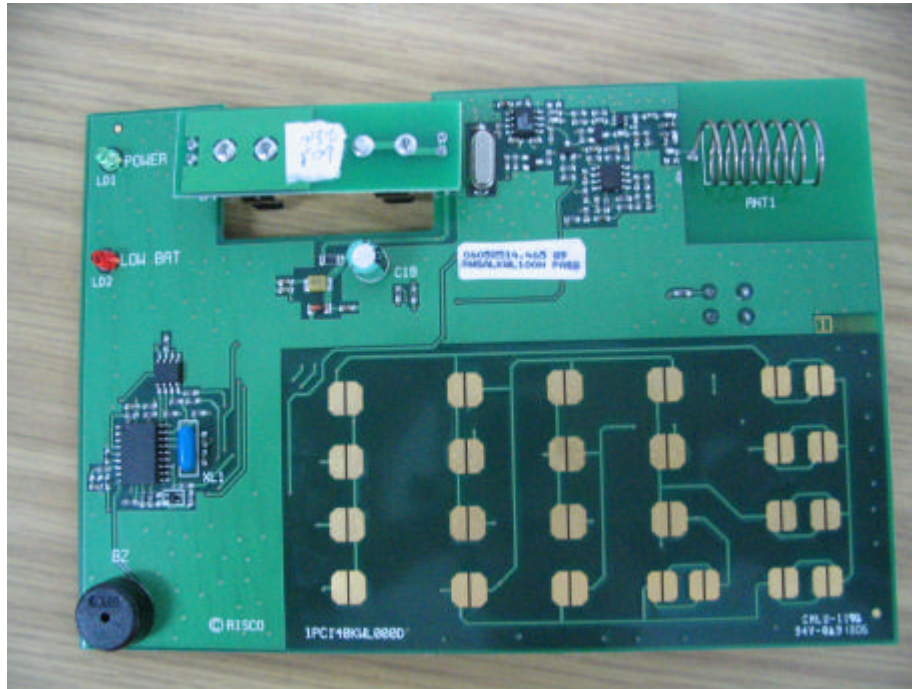
Photograph No.3 Main and RF PCB, first side
