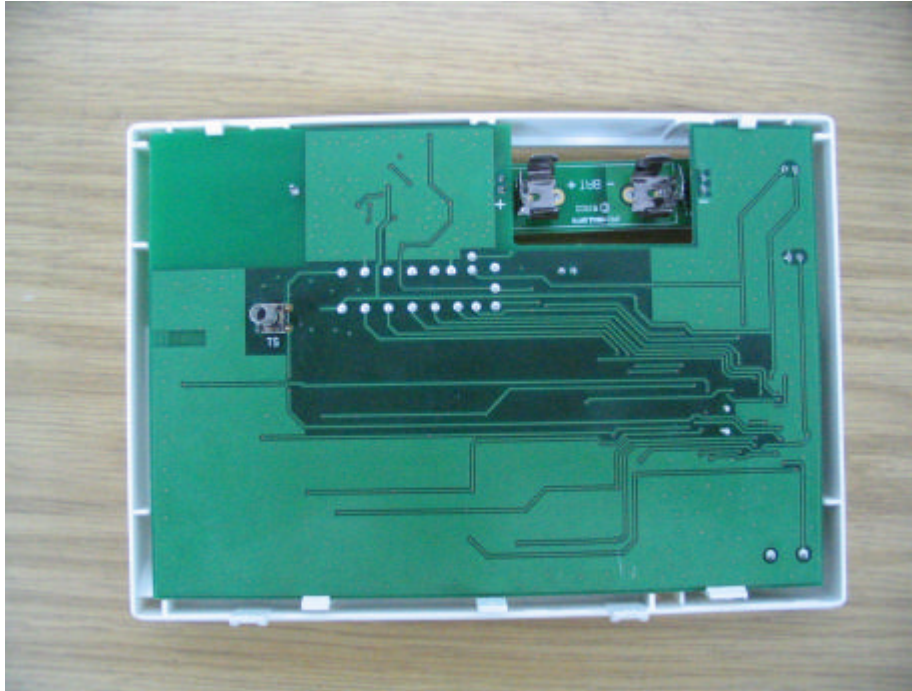
Photograph No.1 RWTSALKWL1USH keypad internal view
