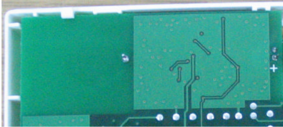
Photograph No.7 Print side of the RF PCB
