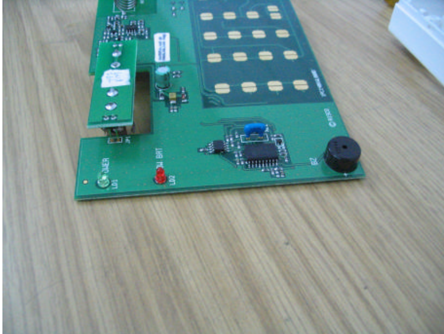
Photograph No.4 Main and RF PCB, first side
