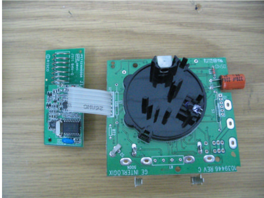
Photograph No.7 Main and RF PCBs, second side
