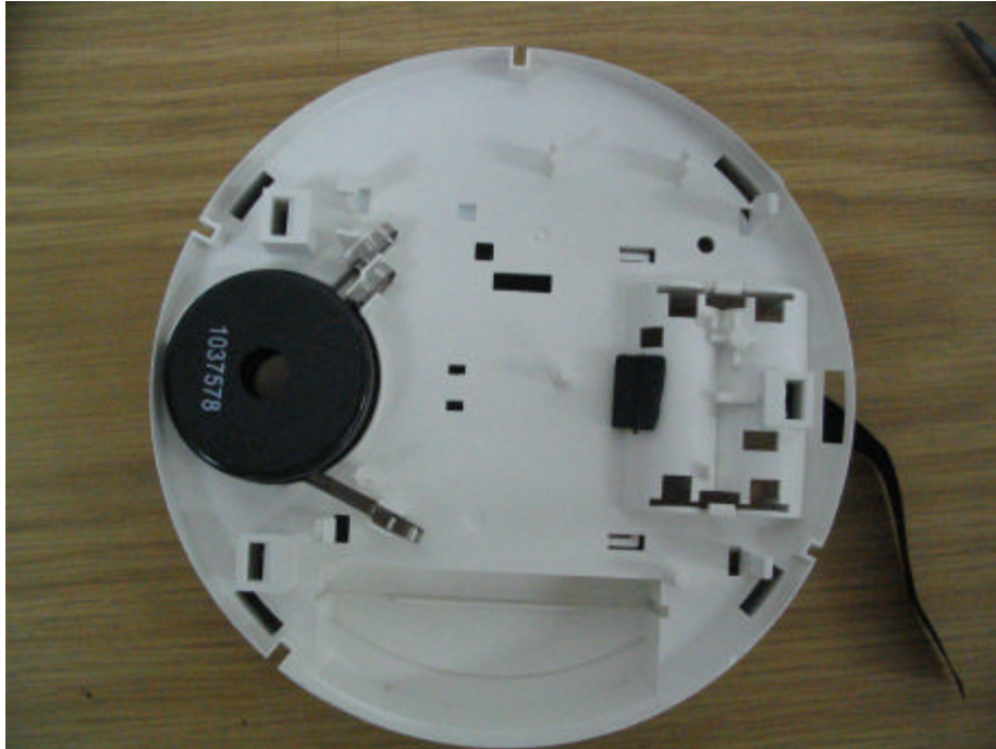
Photograph No.5 RWT30S433USA detector internal view, enclosure
