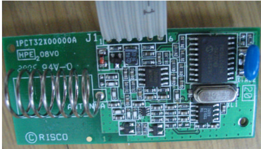
Photograph No.10 Component side of the RF PCB
