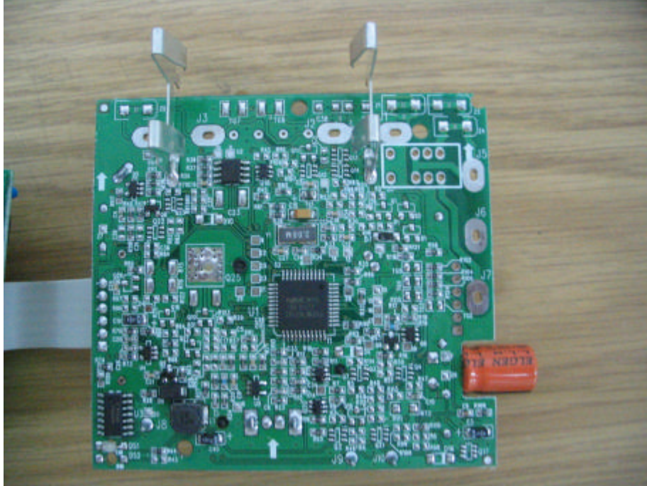
Photograph No.8 Component side of the main PCB
