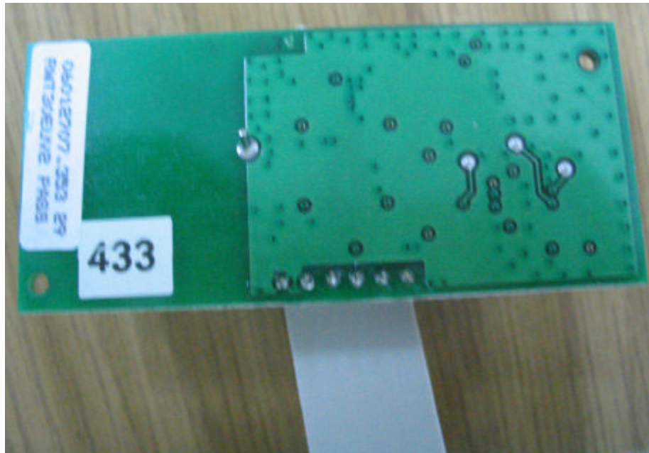
Photograph No.11 Print side of the RF PCB
