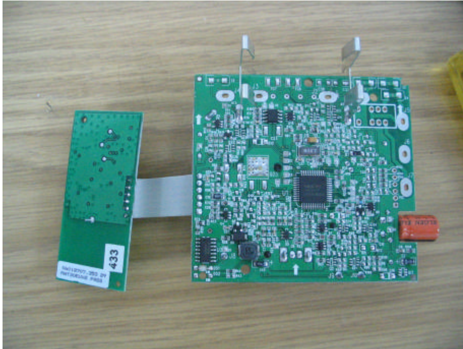
Photograph No.6 Main and RF PCBs, first side
