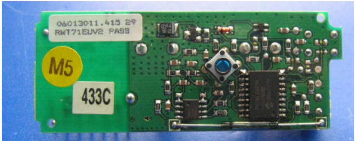
Photograph No2 Print side of the main/RF PCB
