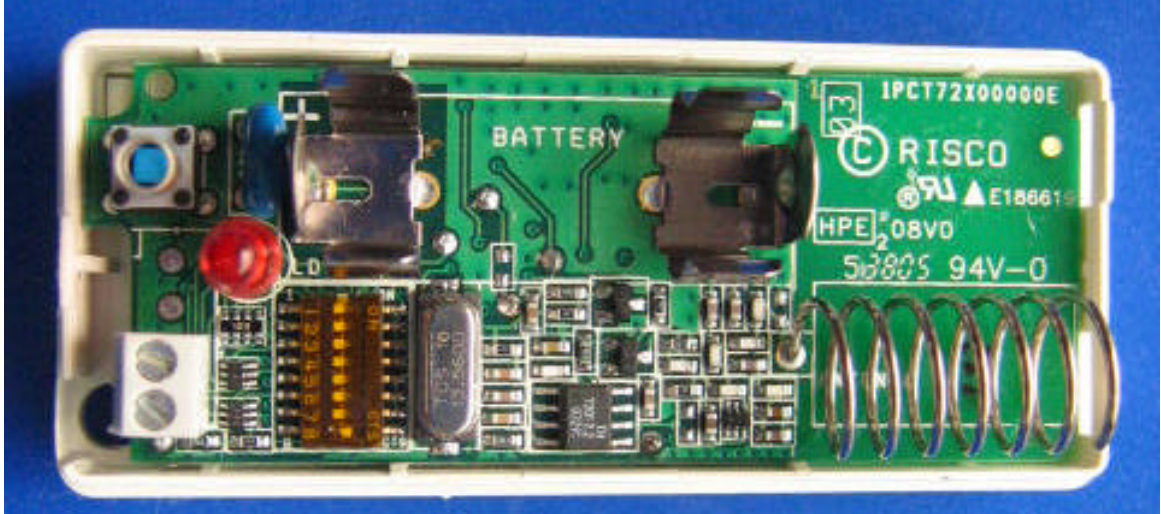
Photograph No.1 Component side of the main/RF PCB
