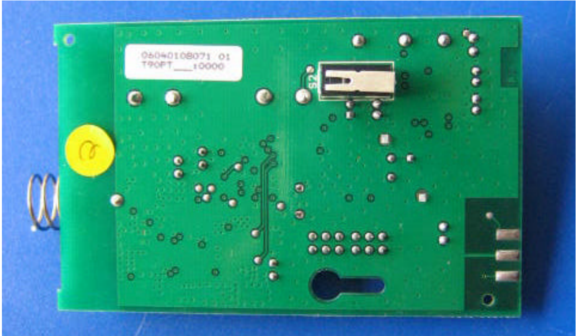
Photograph No.3 Print side of the main/RF PCB
