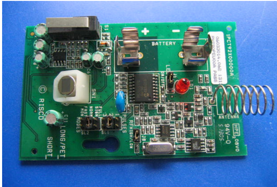
Photograph No2 Component side of the main/RF PCB
