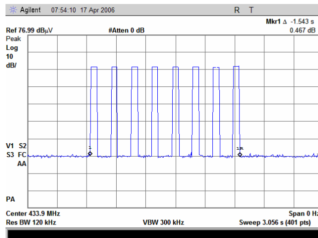
Plot 7.1.2 Number of bursts within one alarm transmission
