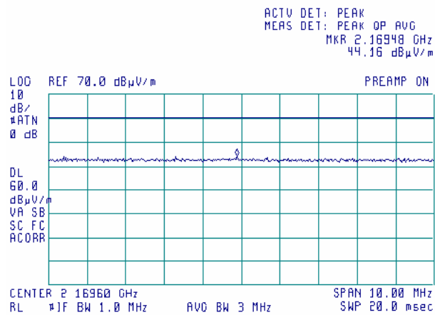
Plot 7.2.13 Radiated emission measurements at the sixth harmonic frequency
