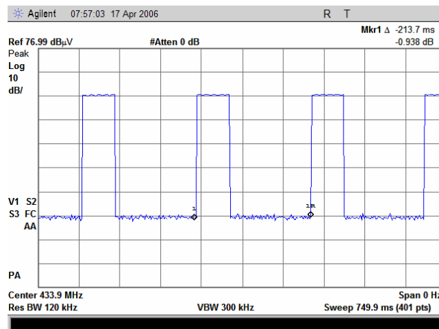
Plot 7.1.4 Burst period
