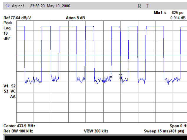
Plot 7.1.6 Pulse duration
