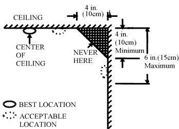
Figure 3: Recommendations for best and acceptable installation locations for installing smoke & heat detectors.
