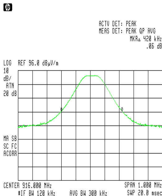
Figure 6 26 dB Bandwidth
