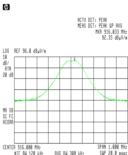
Figure 9. Field Strength of Fundamental. Antenna Polarization: HORIZONTAL. Detector: Peak
