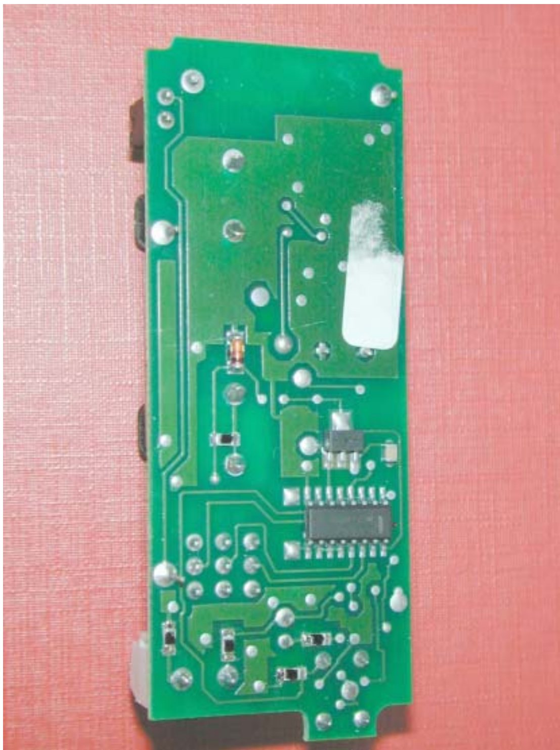
Photograph No.4 RWT71V2 detector PCB second side view
