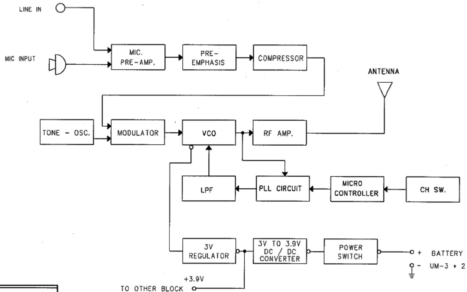
BLOCK DIAGRAM UHF BAND PLL SYSTEM MICROPHONE TRANSMITTER MODEL: DX-837
