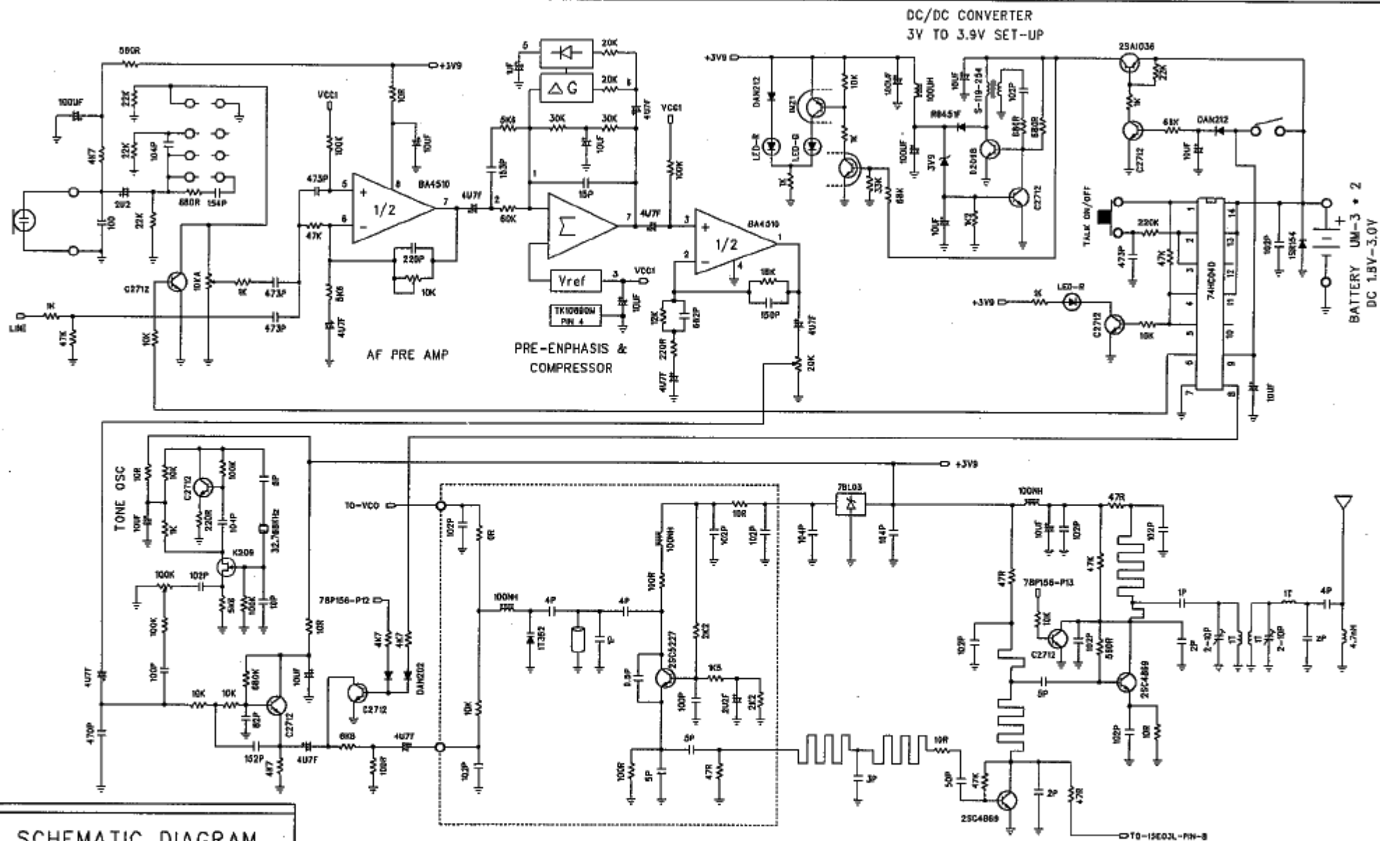
SCHEMATIC DIAGRAM UHF BAND PLL SYSTEM WIRELESS MICROPHONE MODEL : DX-837
