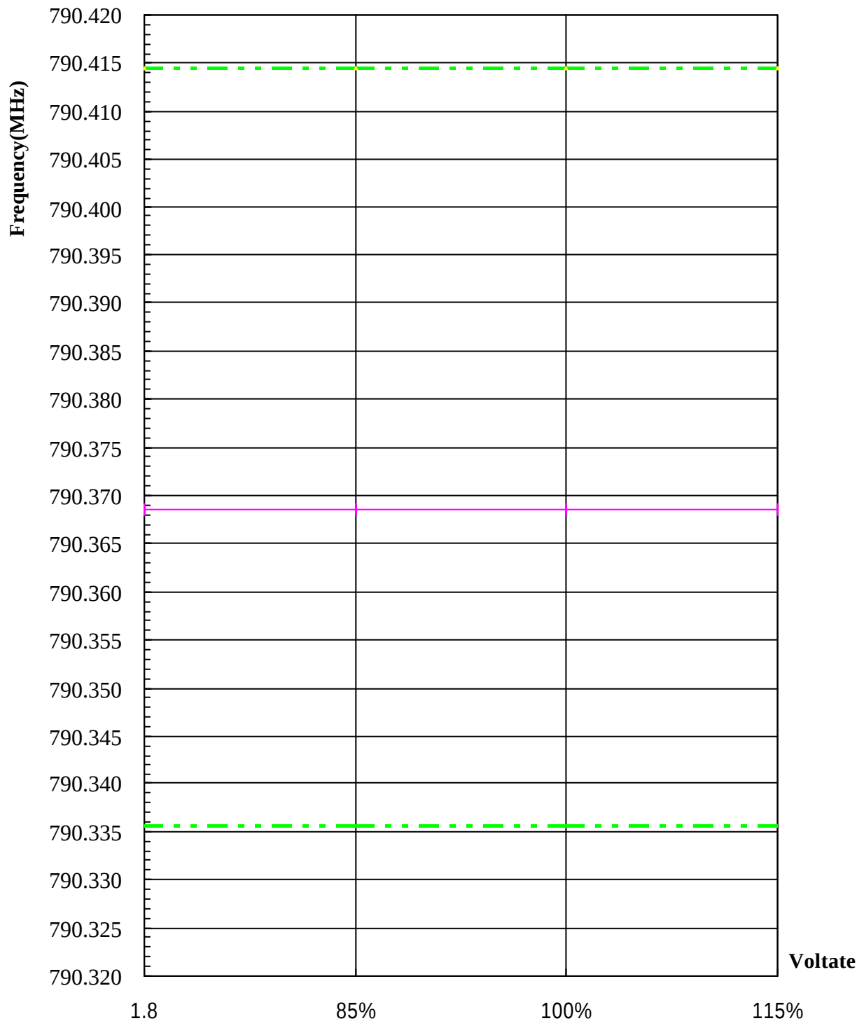
Voltage Variation Vs. Frequency Chart
