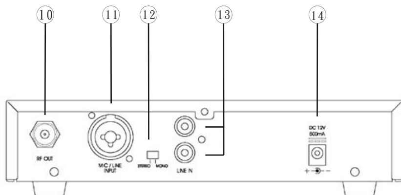
Fig.3 rear panel
