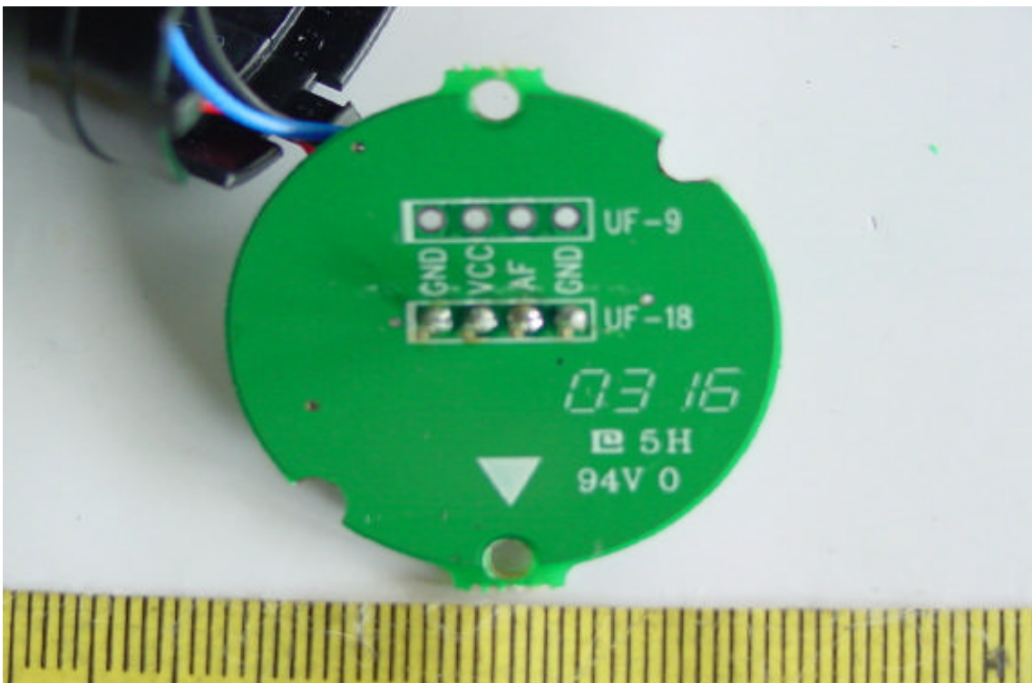
Solder View of PCB 3
