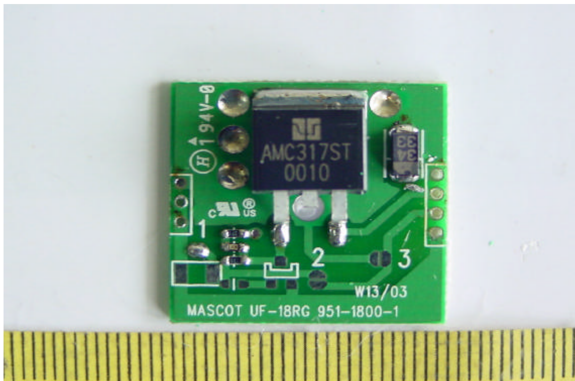
Component View of PCB 2
