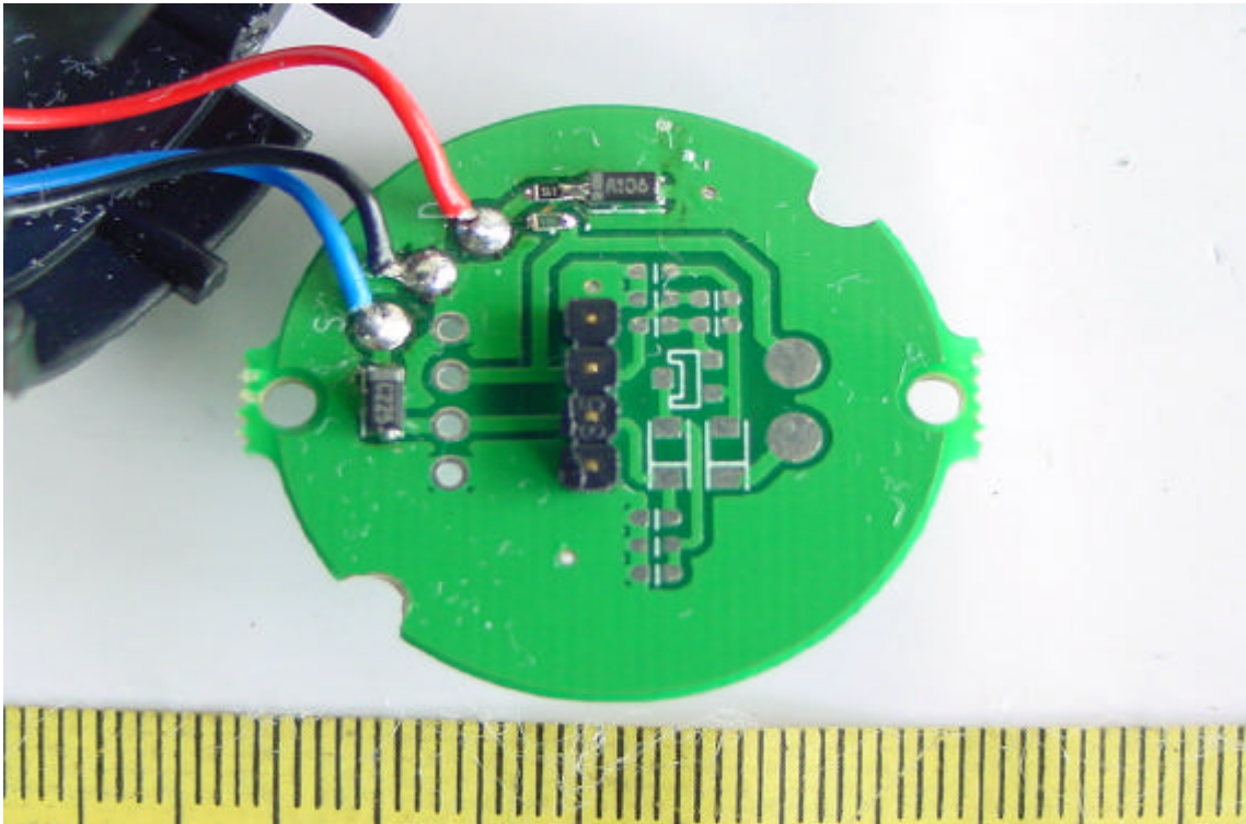
Component View of PCB 3
