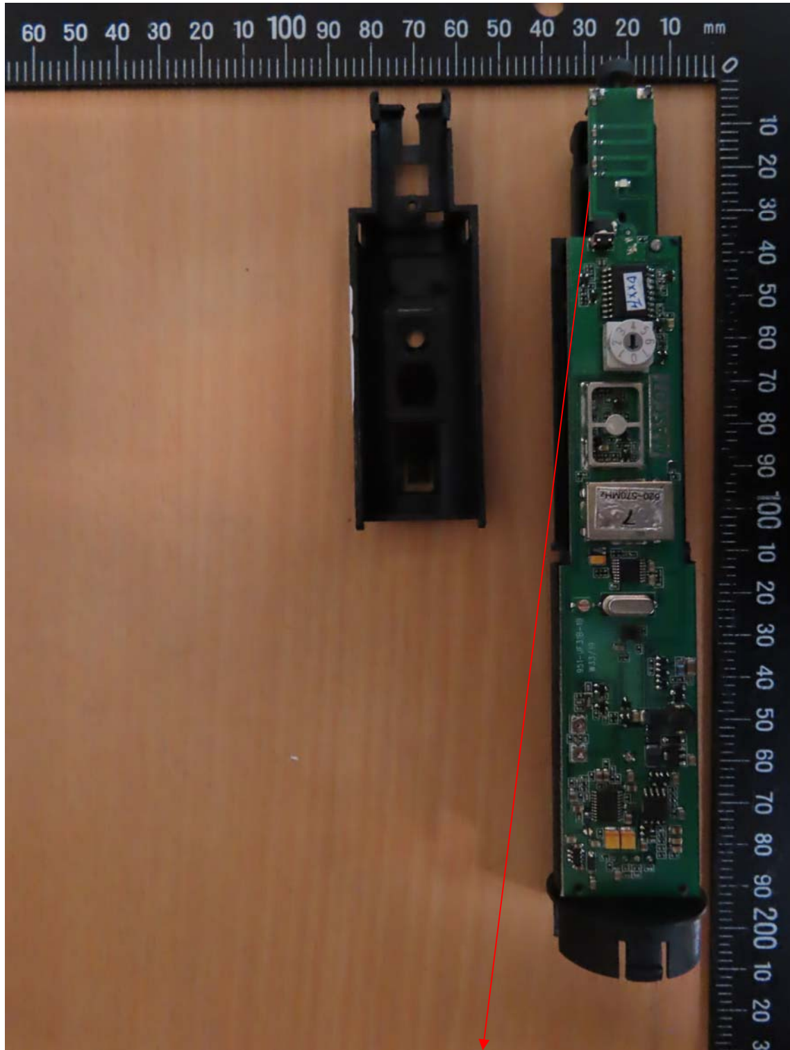
PCB Antenna / Gain: 1.6 dBi
