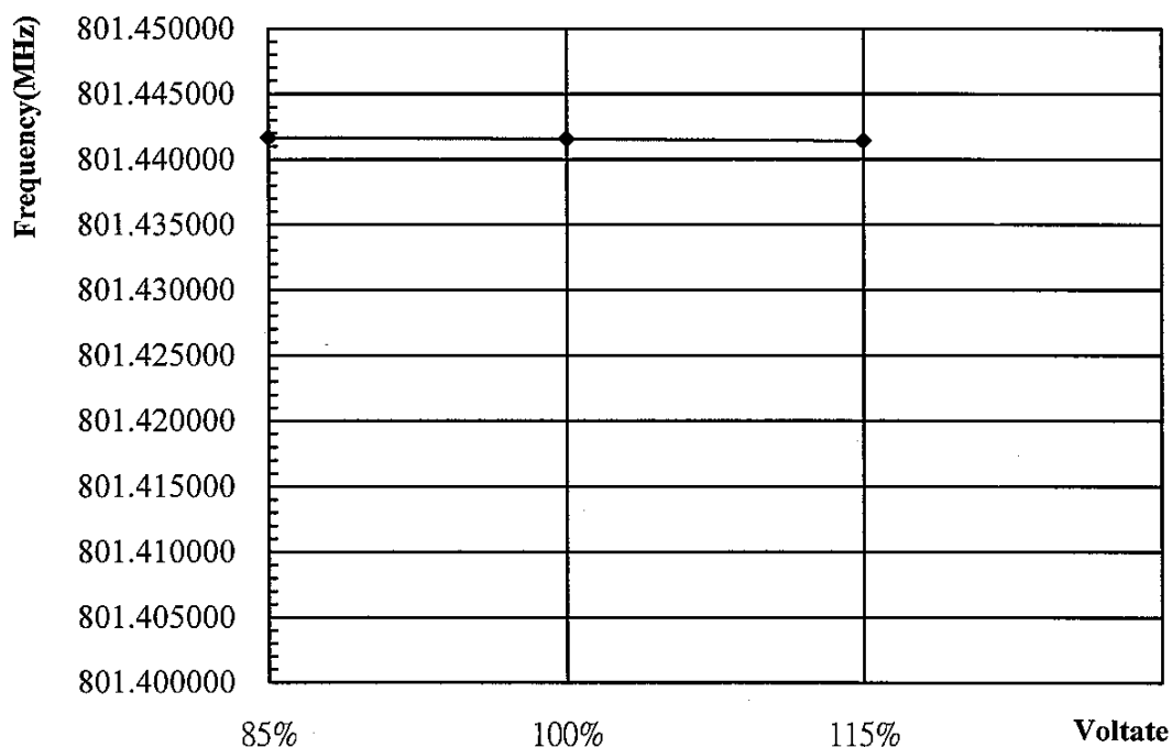
Voltage Variation Vs. Frequency Chart
