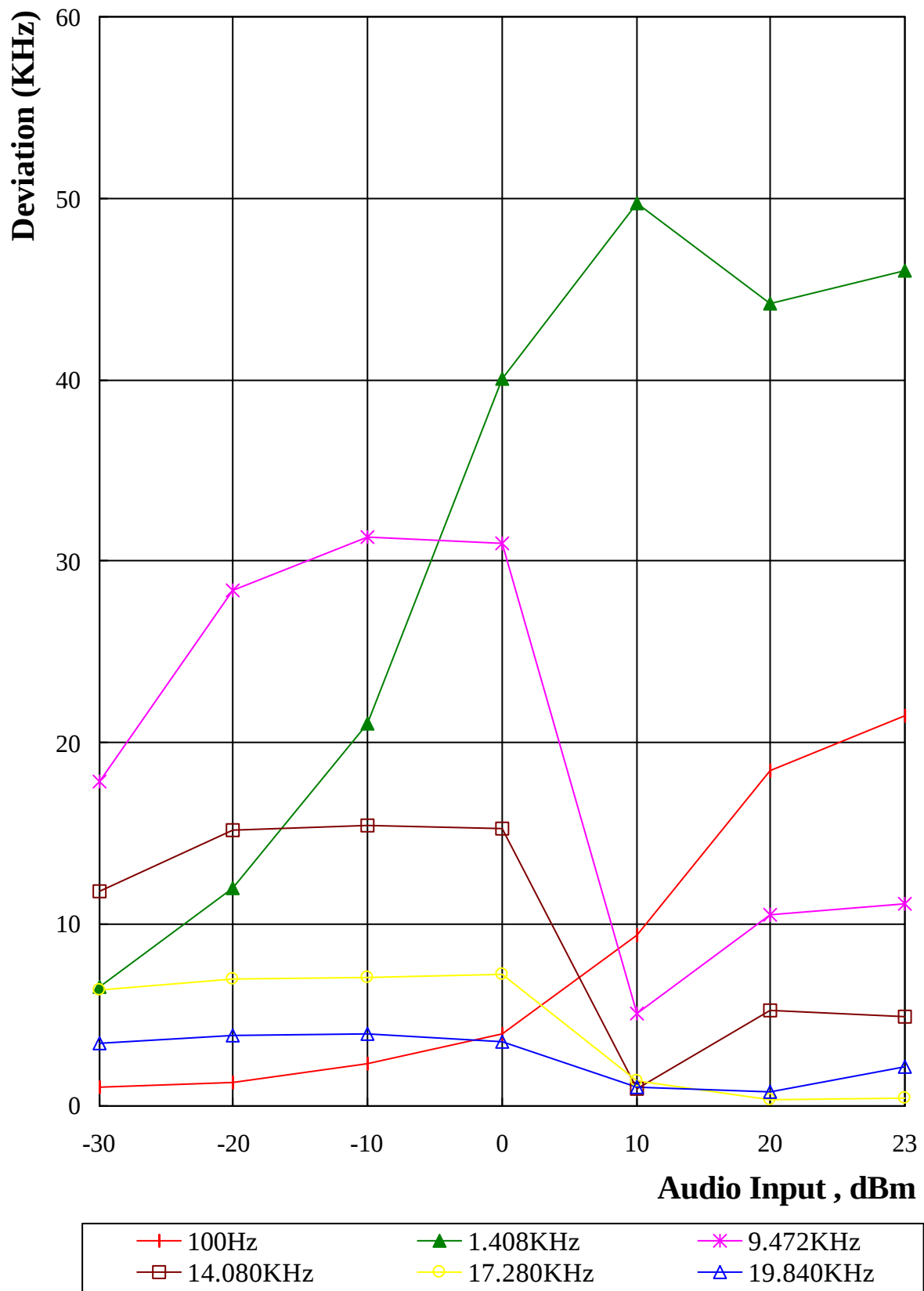
Chart 3.1 Modulation Limiting Measuerment Negative
