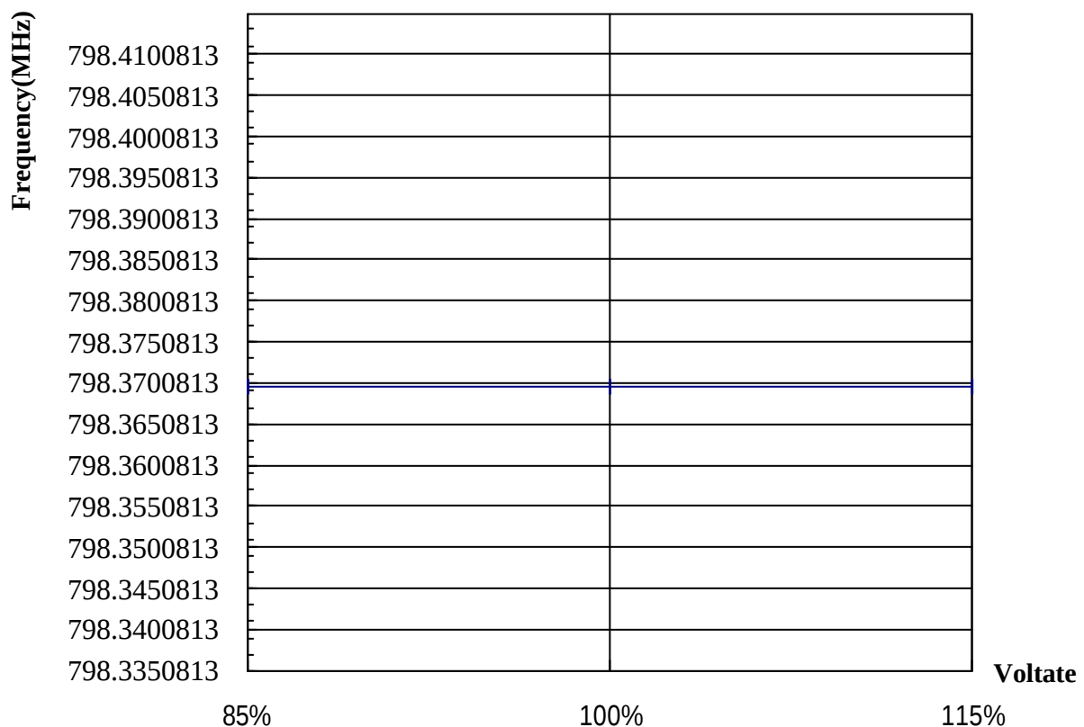
Voltage Variation Vs. Frequency Chart
